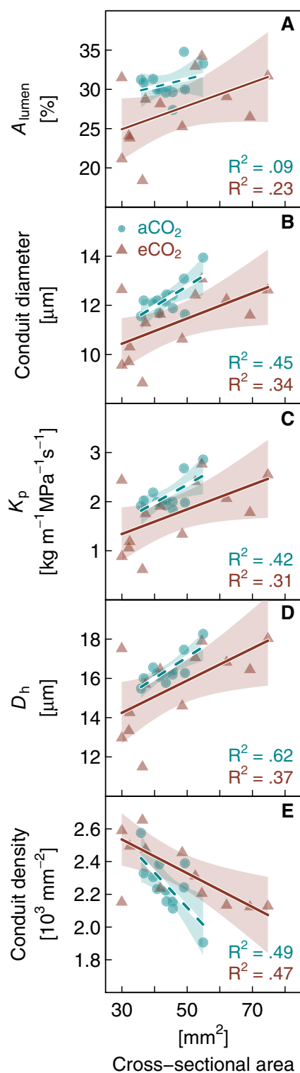
Figure 5 Wood anatomy parameters in relation to branch cross-sectional area in P. halepensis seedlings grown for 40 months under eCO 2 or aCO 2 . A, Lumen fraction ( A_{\text{lumen}} ), (B) average conduit diameter, (C) potential conductivity ( K_p ), (D) hydraulically weighted conduit diameter ( D_h ), and (E) CD are given. Data are measurements of individual branch samples ( n = 12\text{--}13 per treatment). Linear regressions (aCO 2 : intermitted lines, eCO 2 : solid lines) and the 95% confidence intervals of the fit are given (shaded areas). Note that differences between treatments were significant for A_{\text{lumen}} , conduit diameter and K_p (generalized least squares test, P < 0.05 ).
