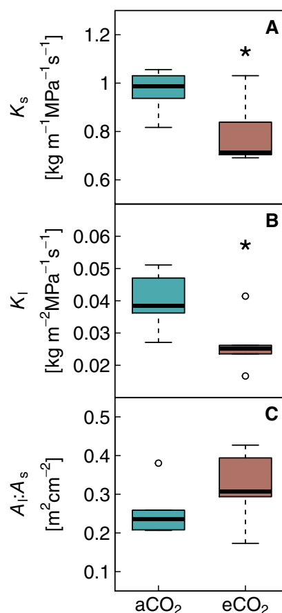
Figure 6 Responses of hydraulic conductivity and leaf-to-sapwood area in 40-month-old P. halepensis seedlings grown under ambient or elevated CO 2 . A, Specific conductivity ( K_s ), (B) leaf specific conductivity ( K_l ), and (C) leaf-to-sapwood area ratio ( A_i:A_s ) are shown as box-plots per treatment ( n = 6 ). The box represents the IQR of the data, the horizontal line inside the box is the median, the whiskers cover 1.5 times the IQR. Data points are outliers beyond the extremes of the whiskers. Significant treatment differences are indicated by asterisks (Mann–Whitney U test P < 0.05 ).
