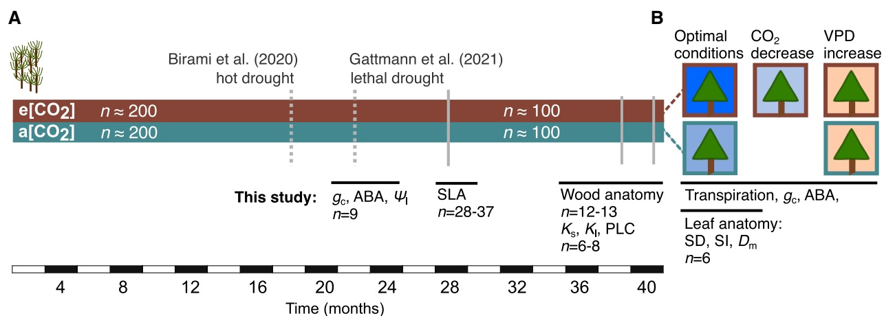
Figure 1 Timeline of cultivation of P. halepensis seedlings under ambient (c. 400 ppm) or (c. 860 ppm) elevated \text{CO}_2 . A, The number of seedlings cultivated after germination, the conducted experiments and references, as well as measurements related to this study are shown. B, After 40 months cultivation, randomly selected seedlings ( n = 6 per treatment) were placed into automated gas exchange chambers enclosing the canopy of one seedling each and transpiration and g_c were measured during optimal conditions, decreasing \text{CO}_2 (in \text{eCO}_2 seedlings only) and increasing VPD over several days alongside which leaf samples were taken to analyze for ABA content. B, This chamber system was also used to measure responses in the same population of seedlings during a dry-down experiment on 22-month-old seedlings when also leaf water potential ( \Psi_l ) was measured as published in Gattmann et al. (2021). Changes in leaf morphology were assessed via analyses of specific leaf area (SLA), SD, SI, and vein-to-epidermis distance ( D_m ). Measurements of wood anatomy included conduit diameter, lumen fraction, and potential hydraulic conductivity. Changes in hydraulic properties were assessed via measurements of specific conductivity ( K_s ), leaf-specific conductivity ( K_l ) and PLC.
