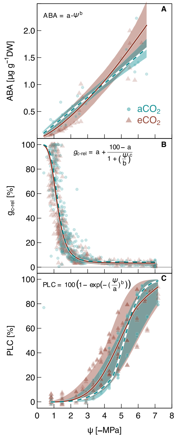
Figure 4 Hydraulic responses to increasing drought in P. halepensis seedlings grown under ambient or elevated \text{CO}_2 . Treatment-specific relationships of (A) leaf-level ABA concentration given per dry weight (DW) needle tissue and (B) relative g_c ( g_{c\text{-rel}} ) with leaf water potential ( \Psi ) during a dry-down experiment are shown for the 22-month-old seedlings ( n = 6 per treatment), and (C) PLC in branches versus xylem water potential ( \Psi ) is given for 40-month-old seedlings (a \text{CO}_2 n = 6 e \text{CO}_2 n = 8 ). Data points of individual measurements (a \text{CO}_2 : solid points, e \text{CO}_2 : solid triangles) are shown. The median of each model is indicated by solid (e \text{CO}_2 ) or dashed (a \text{CO}_2 ) lines and the shaded areas represent the 95% credible intervals per treatment (see Supplemental Table S2 for model coefficients). For values of P_{12} , P_{50} , and P_{88} , see Table 1.
