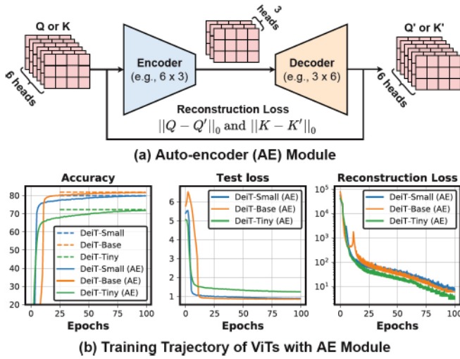
Fig. 9. Illustrating (a) the lightweight and learnable auto-encoder module and (b) the training trajectory of ViTs with such auto-encoder modules, where the dashed lines denote the corresponding vanilla/original ViTs' accuracy without any compression.
