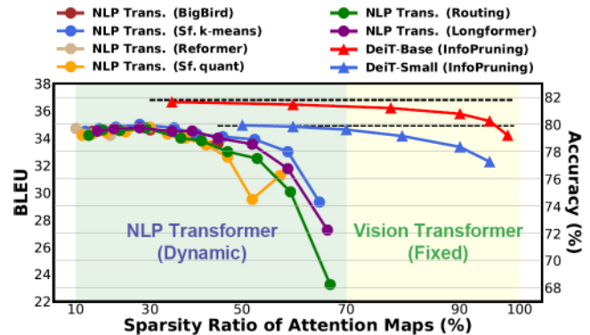
Fig. 1. Comparison between NLP Transformers and ViTs in terms of BLEU-sparsity or accuracy-sparsity trade-offs. Note that for NLP Transformer, we collect the results on machine translation task, IWSLT EN \rightarrow DE, following [39]; For ViTs, we apply an info-based pruning technique on DeiT-Base/Small models and classification task (e.g., ImageNet), following [19].
