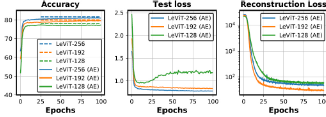
Fig. 18. Training trajectory of LeViTs with AE modules, where dashed lines denote vanilla LeViTs' accuracy.
