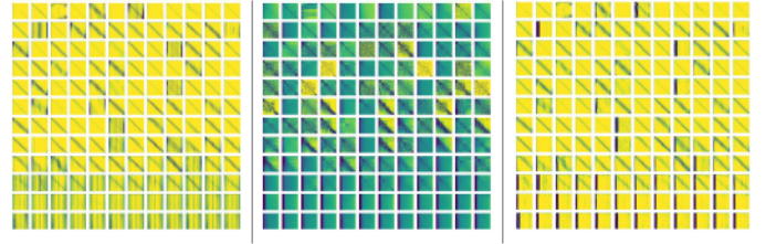
Fig. 8. Visualizing the attention maps of 144 heads (12 layers \times 12 heads) in DeiT-Base after gradually applying our split and conquer algorithm: (a) pruning only; (b) reordering only; (c) both pruning and reordering, where the resolution is 197 \times 197 with 197 being the number of input tokens/patches.
