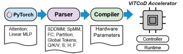
Fig. 14. The algorithm-hardware interface pipeline.
