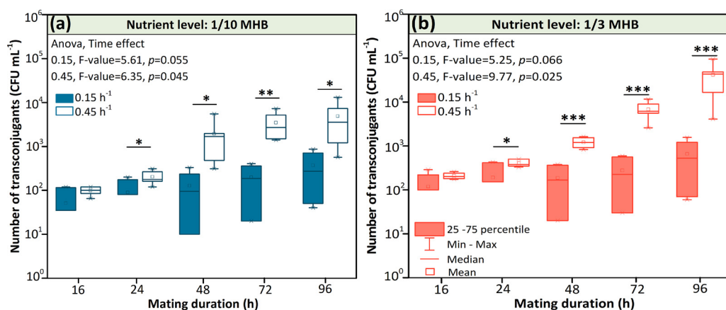
FIG 3 Concentrations of transconjugants ( n = 6 ) at 0.45 \text{ h}^{-1} and 0.15 \text{ h}^{-1} growth rates with nutrient levels of 1/10 MHB (a) and 1/3 MHB (b). Asterisks represent statistically significant differences (i.e., *, **, and *** indicate P < 0.05 , P < 0.01 , and P < 0.001 , respectively [Tukey's post hoc test]).
