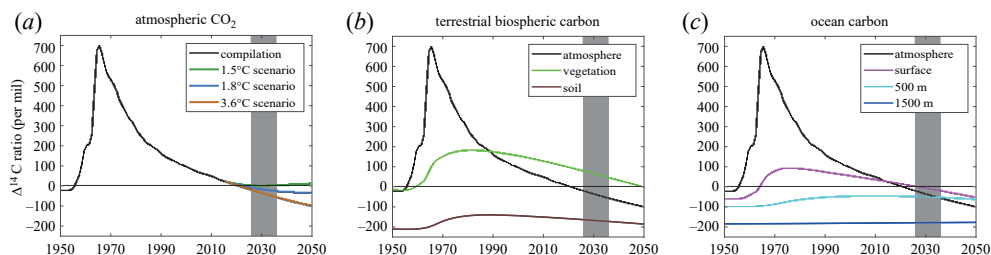
Figure 1. Radiocarbon in the Anthropocene. (a) Measured ^{14}\text{C} ( ^{14}\text{C}/^{12}\text{C} ) in atmospheric \text{CO}_2 between 1950 and 2015 from a compilation [12] together with future projections for the global mean ^{14}\text{C} in three scenarios with different greenhouse gas emissions trajectories and different global average temperatures in 2100 (1.5°C: SSP1–1.9, 1.8°C: SSP1–2.6 and 3.6°C: SSP3–7.0; [3]). The compilation combines various data sources and is representative of tropical regions [12]. Data are reported with typical normalization and correction [13]. (b) Simulated global mean ^{14}\text{C} in terrestrial vegetation and soil carbon and (c) simulated global mean ^{14}\text{C} in ocean carbon at the surface and at 500 m and 1500 m depths from the CESM2 model's historical and SSP3–7.0 experiments of the Large Ensemble (member 1001.001) following CMIP6 protocols [14,15]. Also plotted in (b) and (c) is the ^{14}\text{C} in atmospheric \text{CO}_2 from the compilation and the SSP3–7.0 scenario. In (b) areas poleward of 60° are excluded. The grey vertical bars indicate the proposed International Decade of Radiocarbon.
