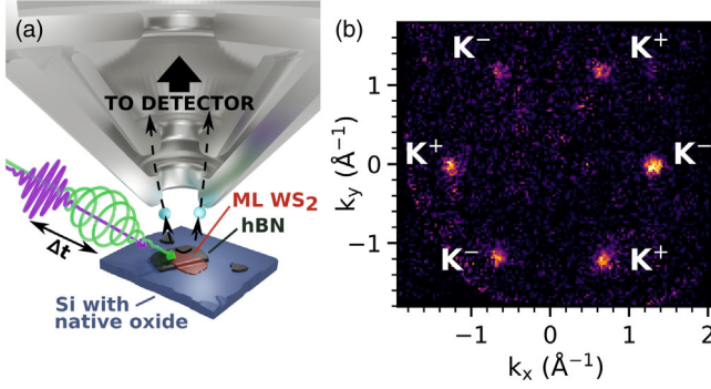
FIG. 1. Time-resolved ARPES of excitons in monolayer \text{WS}_2 . (a) Linearly or circularly polarized pump pulses excite the sample, and a time-delayed XUV probe pulse photojects electrons that are extracted into the momentum microscope. (b) Raw exciton signal at 210 fs delay ( h\nu_{\text{probe}} = 25.2 eV).
