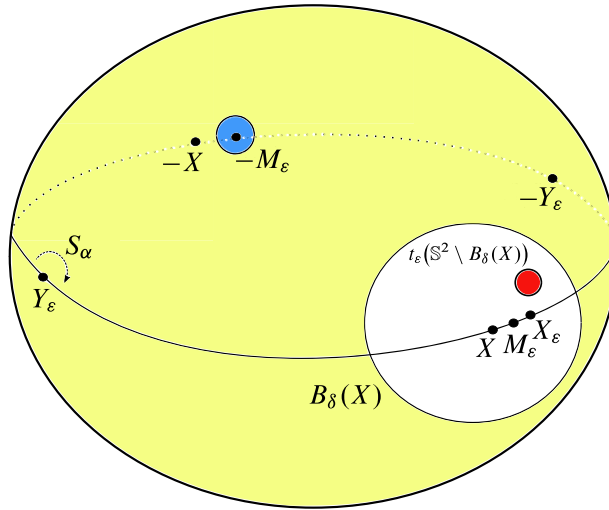
Figure 1. (Color online) The white ball corresponds to B_\delta(X) , the blue ball to A_\varepsilon(\mathbb{S}^2 \setminus B_\delta(X)) , and the red ball to t_\varepsilon(\mathbb{S}^2 \setminus B_\delta(X)) .
