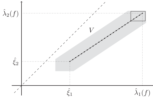
FIGURE 3. Illustration of the proof of Theorem 1.5 with d = 3 , u = 1 . The function g_u \circ T^{-1} is positive on the sector between the horizontal positive semi-axis and the diagonal. The gray region is the neighborhood V , and the marked points along the segment [\hat{\xi}, \hat{\lambda}(f)] are the \eta_i values. For the first perturbation (g_{0,t}) , the corresponding hatted Lyapunov vector \hat{\lambda}(g_{0,t}) stays inside the upper right rectangle and hits \eta_1 for some parameter t = t_0 .
