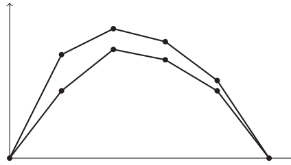
FIGURE 1. The top graph shows j \in \{0, \dots, d\} \mapsto \hat{\lambda}_j(f) for some f . The bottom graph corresponds to T(\xi) for some ordered vector \xi satisfying assumptions (a)–(b) from Theorem 1.5.
