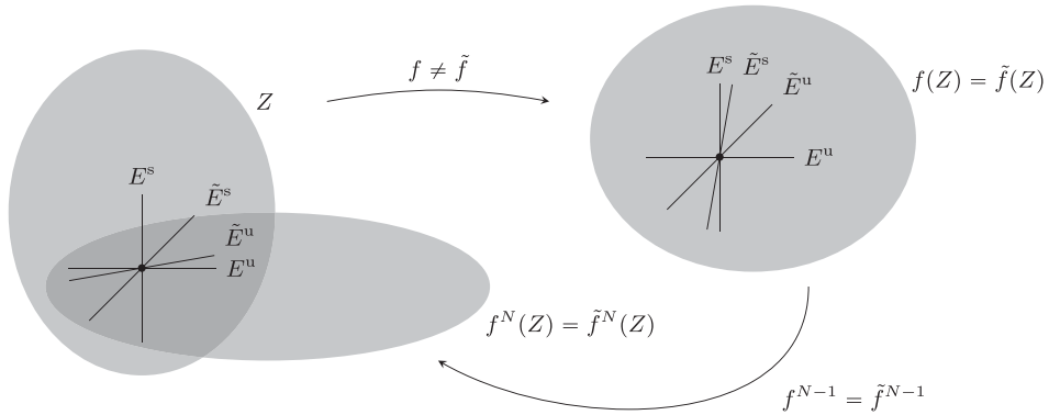
FIGURE 4. A damping perturbation \tilde{f} of an Anosov diffeomorphism f .
