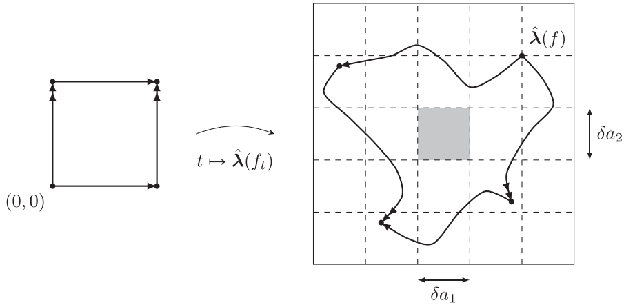
FIGURE 2. Illustration of Proposition 2.1 for d = 3 . The images of the edges of the square [0, 1]^2 under the map t \mapsto \hat{\lambda}(f_t) stay on the strips determined by conditions (2.4) and (2.5). Corollary 2.2 tells us that the image of this map is a set \Lambda that contains the small gray square and is contained in the big square.
