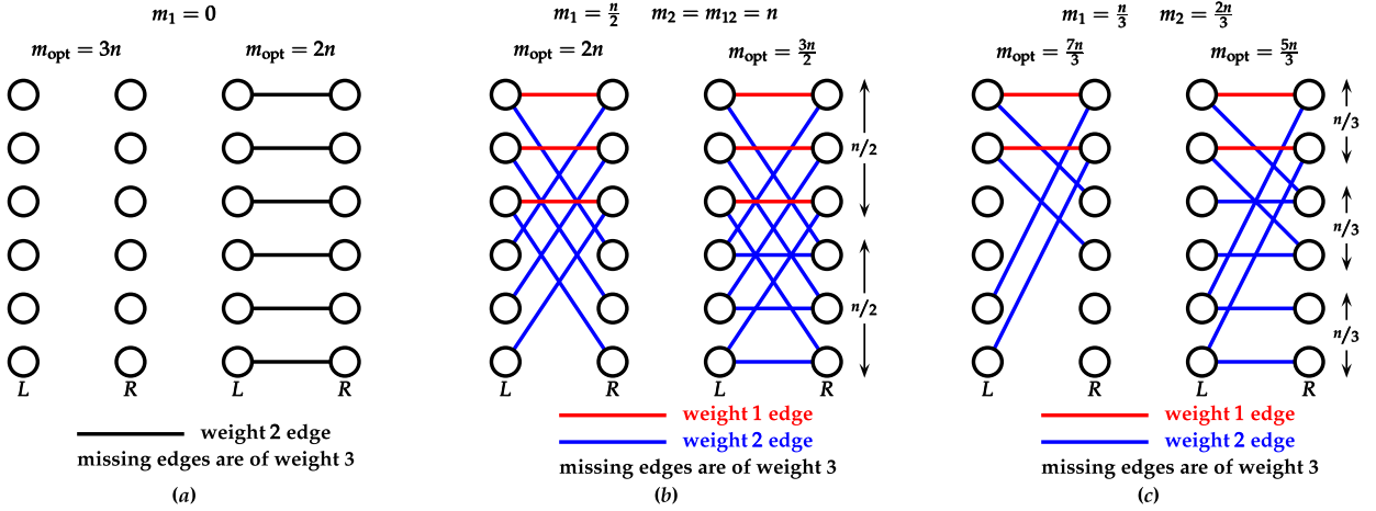
Fig. 1. (a) Example showing tightness of bounds in Theorem 5 when only estimate for m_1 is known. (b) Example showing tightness of bounds in Theorem 5 when estimates for m_1, m_2, m_{12} are known. (c) Example showing that better than additive \frac{2}{3} -approximation is not possible if only estimates for m_1 and m_2 are used for the case in Theorem 5(b).
