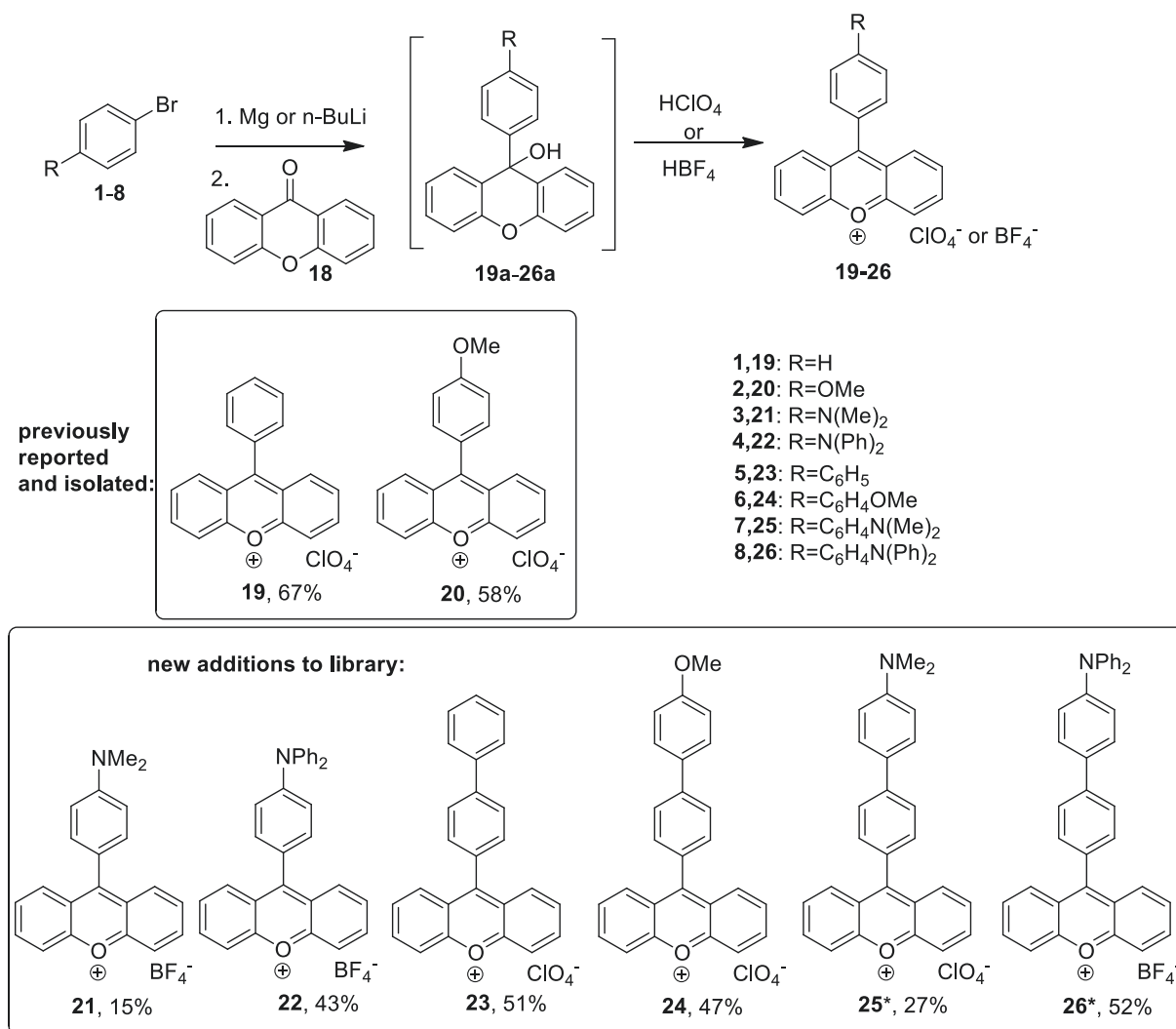
Scheme 2. General Synthesis of Expanded Library of 9-aryldibenzo[b,e]pyrylum (xanthylum) salts.
