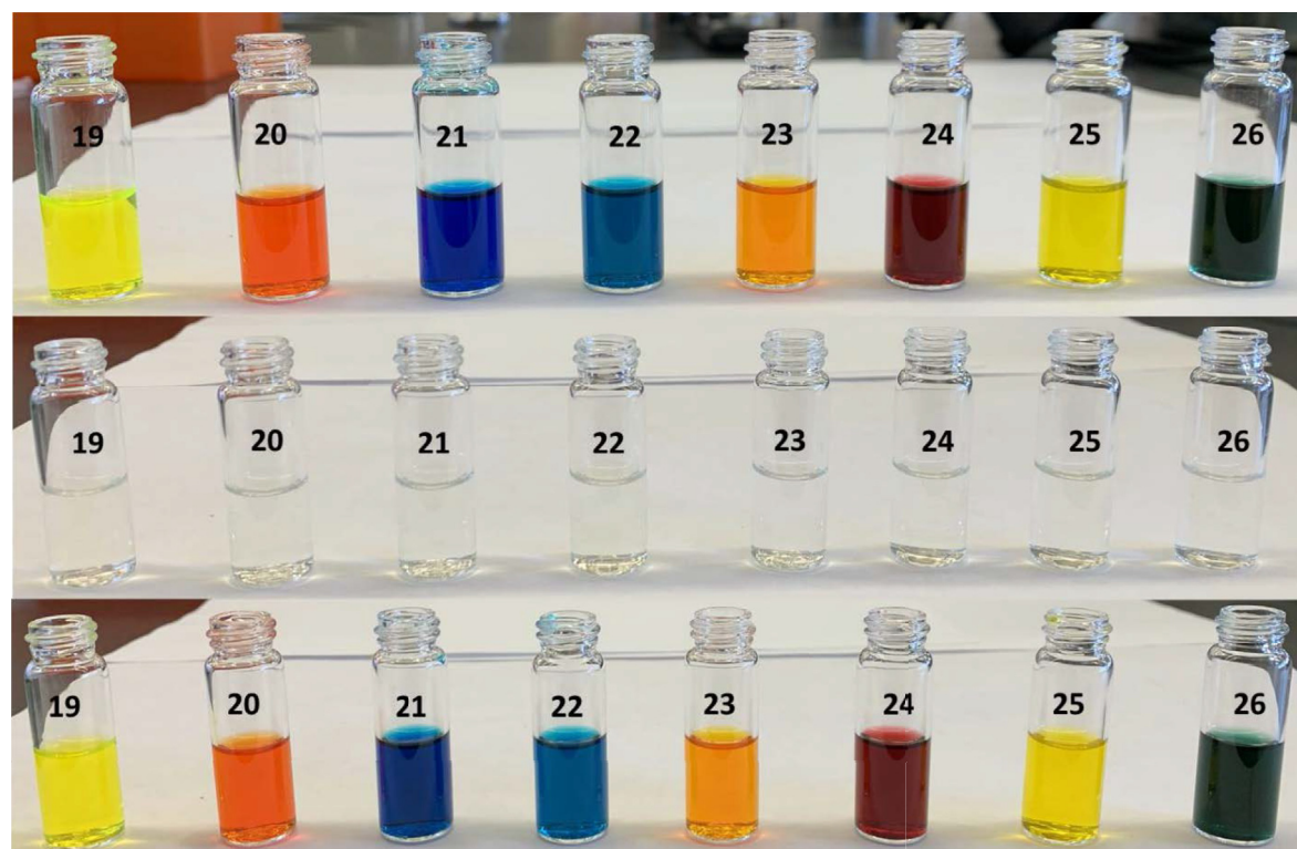
Fig. 3. Photographs of 9-aryldibenzo[b,e]pyrylium salts 19–26 in solution. Top: Vials containing 2 mL solutions of 19–26 , 1.0 mM in CH 3 CN. Middle: Vials from the top after addition of 80 µL of TEA. Bottom: Vials from the middle after addition of 200 µL of TFA.
