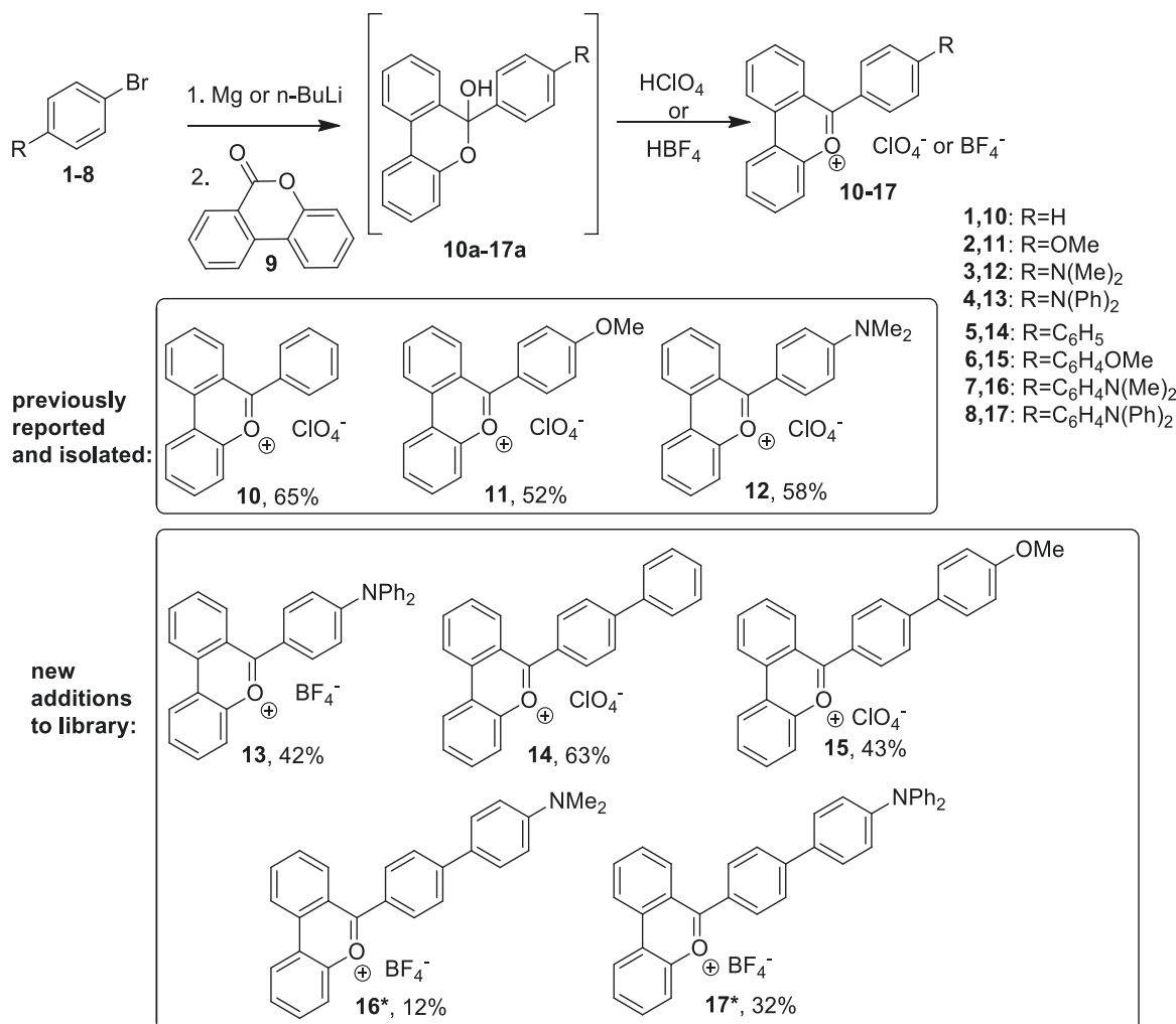
Scheme 1. General Synthesis of Expanded Library of 6-aryldibenzo[b,d]pyrylium salts.
