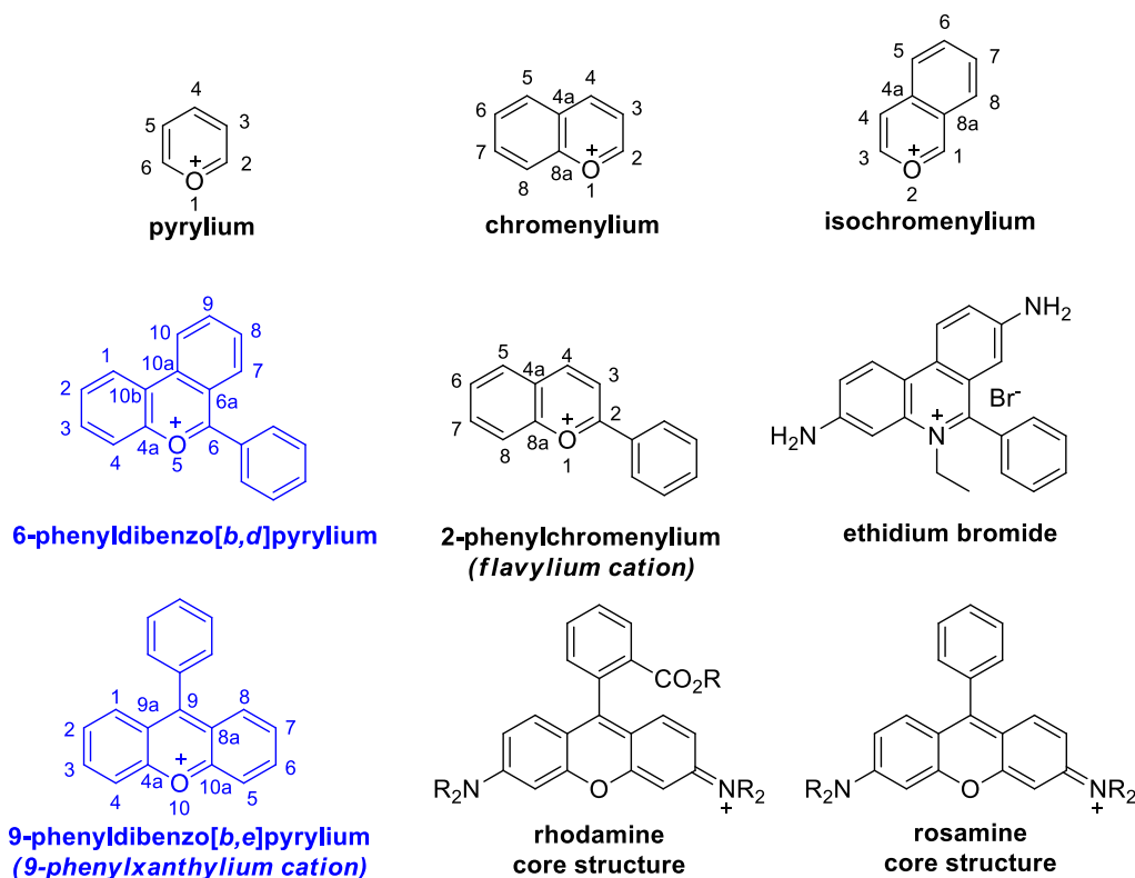
Fig. 1. Structures of different cationic aromatic pyrylium-based heterocycles and their derivatives.
