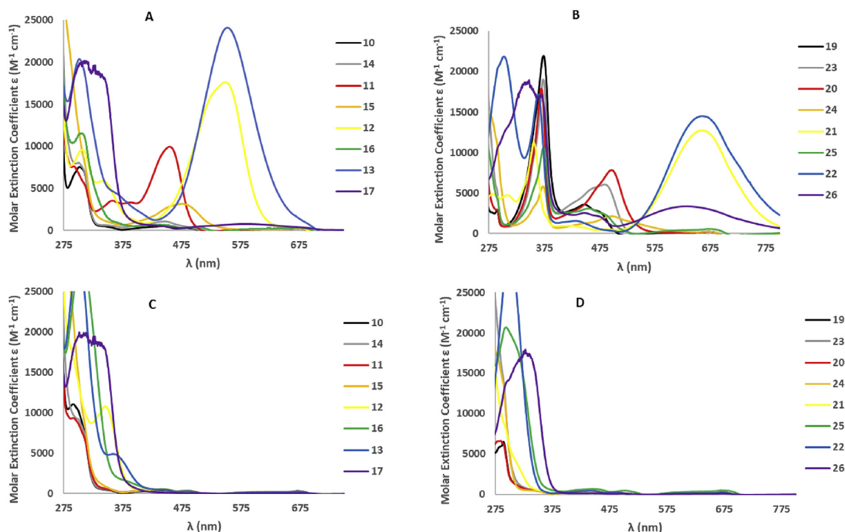
Fig. 4. UV–vis spectra for: (A) 10–17 30.0 \mu\text{M} in \text{CH}_3\text{CN} ; (B) 19–26 30.0 \mu\text{M} in \text{CH}_3\text{CN} ; (C) samples from (A) after addition of 1 drop of TEA; (D) samples from (B) after addition of 1 drop of TEA.
