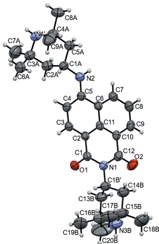
Figure 1 The asymmetric unit of bis -TMP naphthalimide represented with displacement ellipsoids at the 50% probability level and disordered TMP omitted for clarity.
