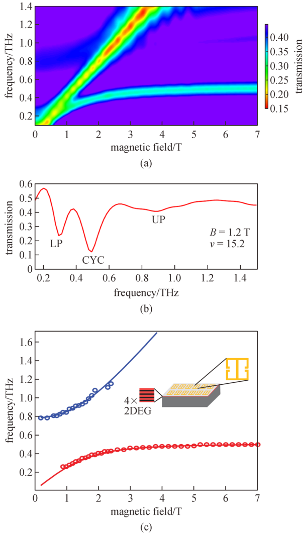
Fig. 7 Ultrastrong coupling between THz split-ring resonators and the CR of a high-mobility 2DEG. (a) Transmission as a function of B at 10 K. (b) A vertical cut from panel (a) in the anticrossing region at B = 1.2 T. Both the upper-polariton and lower-polariton modes are observed together with the free-space CR (CYC) arising from the uncovered regions of the 2DEG. (c) Polariton branches plotted as a function of magnetic field. Solid lines are theoretical calculations. Inset: schematic of the 500 GHz resonator deposited on the sample surface. Adapted from Ref. [55]
