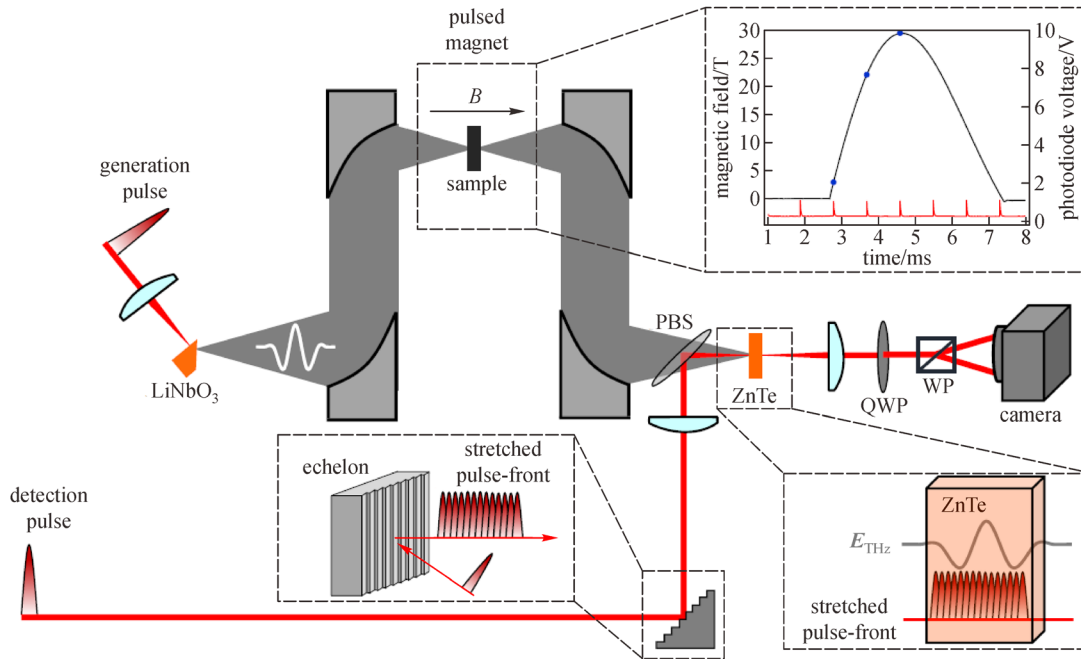
Fig. 3 Free-space single-shot THz time-domain spectroscopy system combined with a pulsed magnet [41,42]. THz pulses strong enough for single-shot detection are generated using LiNbO 3 . Detection is performed in a single-shot manner using a reflective echelon, which stretches the probe pulse in the time domain. The inset at the top shows that for a 1-kHz repetition-rate laser, three measurements can be done on the rising edge of the magnetic field pulse. A pellicle beamsplitter (PBS) is used to combine the THz and near-infrared probe beams. A quarter-wave plate (QWP) and a Wollaston prism (WP) are commonly used to detect the polarization rotation of the probe beam
