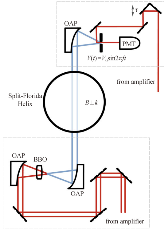
Fig. 2 Free-space THz time-domain spectroscopy system combined with the Split-Florida Helix Magnet [68]. The broadband THz pulses are generated by mixing the fundamental and its second-harmonic laser field (generated from a frequency-doubling BBO crystal) in a nitrogen-purged atmosphere. Laser pulses are focused and collimated using off-axis parabolic (OAP) mirrors. The THz wavevector is perpendicular to the applied magnetic field (Voigt geometry). For detection, THz pulses are focused onto a THz-air breakdown coherent detector (THz-ABCD). A portion of the fundamental beam is used to gate the THz-ABCD to recover the full electric field waveform
