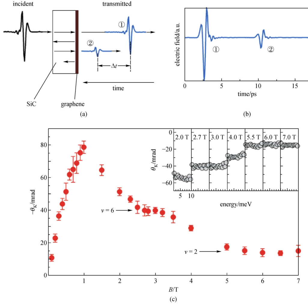
Fig. 5 Magneto-optical Kerr rotation in monolayer graphene. (a) Schematic of the experimental configuration depicting the transmission of a THz pulse through the sample. (b) Time-domain waveform of the THz pulse transmitted through the sample. (c) Magnetic field dependence of the Kerr rotation at 1 THz for the sample with a Fermi energy of 70 meV. The inset shows Kerr rotation spectra at the indicated magnetic fields. Adapted from Ref. [116]
