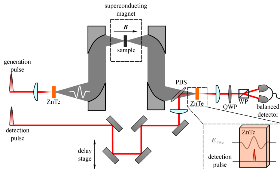
Fig. 1 Free-space THz time-domain spectroscopy (THz-TDS) system combined with a superconducting magnet. The generation and detection of THz radiation is achieved via optical rectification and the electro-optic effect, respectively, using ZnTe crystals. A pellicle beamsplitter (PBS) is used to combine the THz and near-infrared probe beams. A quarter-wave plate (QWP) and a Wollaston prism (WP) are commonly used to detect the polarization rotation of the probe beam
