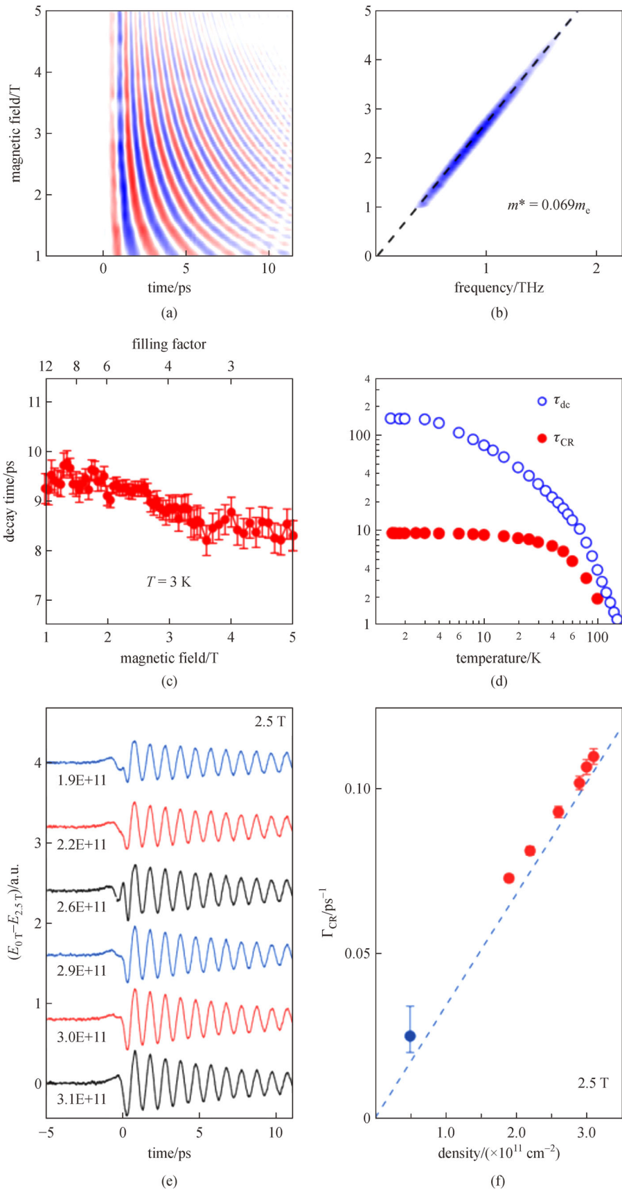
Fig. 4 Superradiant decay of cyclotron resonance in ultrahigh-mobility two-dimensional electron gases [63]. (a) Magnetic field dependence of CR oscillations in the time domain, showing peaks (blue) and valleys (red). (b) Frequency-domain version of (a). Black dashed line: a linear fit with a cyclotron mass of 0.069m_0 . (c) Magnetic field dependence of the CR decay time, \tau_{CR} at 3 K. (d) Temperature dependence of \tau_{CR} at 2.5 T and the DC scattering time, \tau_{DC} , determined from the DC mobility, \mu = e\tau_{DC}/m^* . (e) CR oscillations in the time domain for samples with different densities by controlling the illumination time. (f) CR decay rate as a function of electron density. Blue solid circle: sample 2 (low density). Red solid circles: sample 1 (high density). The blue dashed line represents a theoretical relation expected from the phenomenon of superradiance [102] without any adjustable parameter (with n_{\text{GaAs}} = 3.6 and m^* = 0.069m_0 )
