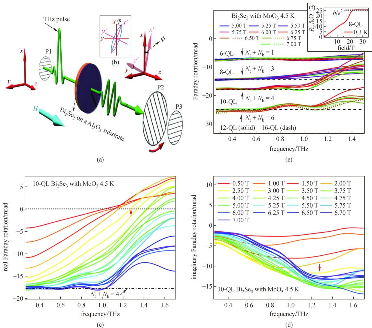
Fig. 6 Quantized Faraday rotation of topological surface states in Bi 2 Se 3 . (a) Schematic diagram of the Faraday rotation experimental setup. P1, P2, and P3 are polarizers. The polarization acquires an ellipticity simultaneously, as shown in (b). (c) Real part of the Faraday rotation of 10-QL Bi 2 Se 3 films with MoO 3 at 4.5 K at various magnetic fields [color-coded as in (d)]. The dash-dotted line is the theoretical expectation. (d) Imaginary part of the Faraday rotation. A representative cyclotron frequency is marked by a red arrow for data at 2.5 T. (e) Quantized Faraday rotation for different samples. Dashed black lines are theoretical expectation values assuming certain values for the filling factor of the surface states. (f) DC Hall resistance of a representative 8-QL sample. Adapted from Ref. [58]
