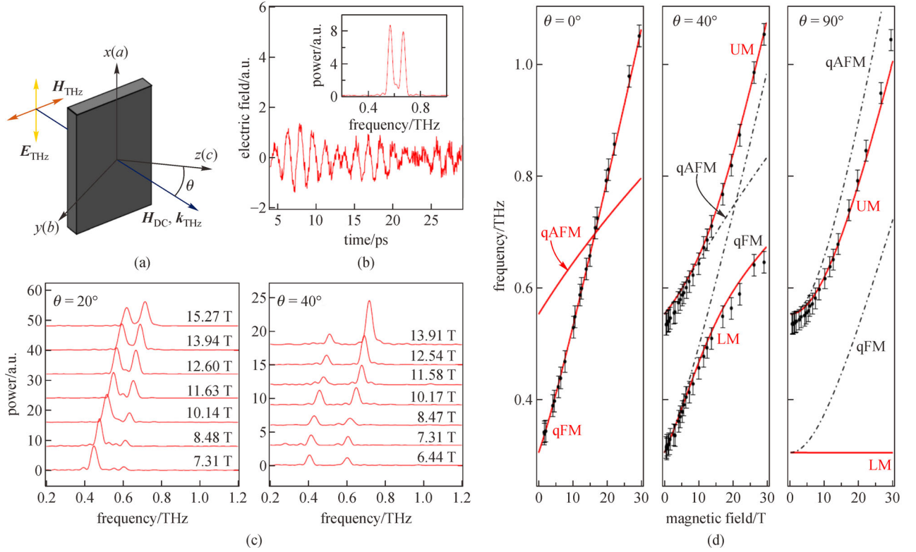
Fig. 9 THz-TDS of magnon-magnon ultrastrong coupling in \text{YFeO}_3 evidencing dominant vacuum Bloch–Siegert shifts [42]. (a) Schematic of THz magnetospectroscopy studies of \text{YFeO}_3 in a tilted magnetic field. H_{DC} was applied in the b – c plane at an angle of \theta with respect to the c -axis, with k_{THz} \parallel H_{DC} and H_{THz} polarized in the b – c plane. (b) Transmitted THz waveform for \theta = 20^\circ at \mu_0|H_{DC}| = 12.60 T displaying beating in the time domain and two peaks in the frequency domain. (c) Magnon power spectra for \theta = 20^\circ and \theta = 40^\circ at different H_{DC} , displaying larger frequency splitting for larger \theta . (d) Experimentally measured magnon frequencies for \theta = 0^\circ, 40^\circ, 90^\circ versus \mu_0|H_{DC}| (black dots) with calculated resonance magnon frequencies (solid red lines) and decoupled qFM and qAFM magnon frequencies (black dashed-dotted lines). The upper mode frequency becomes lower than the qAFM frequency at \theta = 90^\circ , indicating a dominant vacuum Bloch–Siegert shift compared to the vacuum Rabi splitting-induced shift
