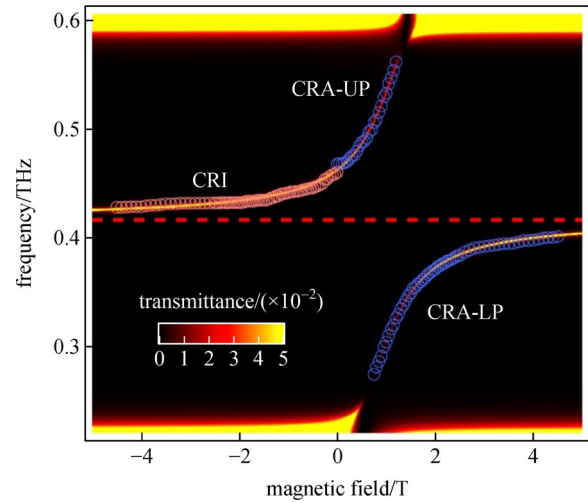
Fig. 8 Vacuum Bloch–Siegert shift in Landau polaritons with ultrahigh cooperativity [65]. Transmission spectra in the vicinity of the anticrossing region between CR and the first cavity mode (red dashed line) for simulations using the full Hamiltonian (solid lines) is shown. The counter-rotating and A^2 terms have to be included in the full Hamiltonian. Experimental data points are shown as open circles
