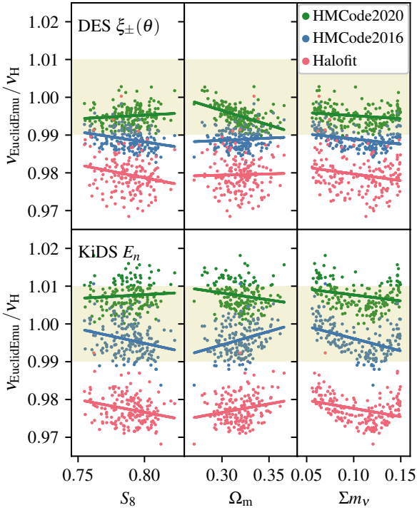
Figure 17. Comparison of the DES \xi_{\pm}(\theta) (upper) and KiDS E_n(\theta_{\text{min}}=0.5) (lower) cosmic shear predictions from HMCODE2020 (green), HMCODE2016 (blue) and HALOFIT (pink), as a ratio with the prediction from the EUCLIDEMULATORV2 (see Equation E1) for a range of cosmological parameters. Each data point represents one sample from the DES Y3 3 \times 2 pt posterior that lies within the allowed parameter range of the EUCLIDEMULATORV2. The solid lines show an unweighted linear best fit to the data points as a function of input S_8 (left), \Omega_m (middle) and \Sigma m_V (right). Only weak trends are seen with all the parameters including those not shown here. The shaded region brackets \pm 1\% accuracy.
