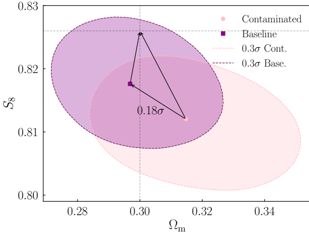
Figure 10. Cosmological constraints in the \Omega_m - S_8 plane from a mock DES-like joint-survey analysis of data vectors from a dark-matter only Universe (‘Baseline’, purple), and an OWLS-AGN baryon-feedback contaminated Universe (‘Contaminated’, pink), for an input cosmology \Omega_m = 0.3 and S_8 = 0.826 (grey-dashed). The contours are set at 0.3\sigma_{2D} , where \sigma_{2D} is the 68% credible interval in the 2D marginalised posterior. In this analysis the KiDS COSEBIs data vector has been created with an increased minimum angular scale of \theta_{\min} = 2'.0 , leading to an offset from the Baseline dark-matter only case of 0.18\sigma_{2D} . We discuss the projection effects that impact both the Baseline and Contaminated analysis in Appendix C.3.
