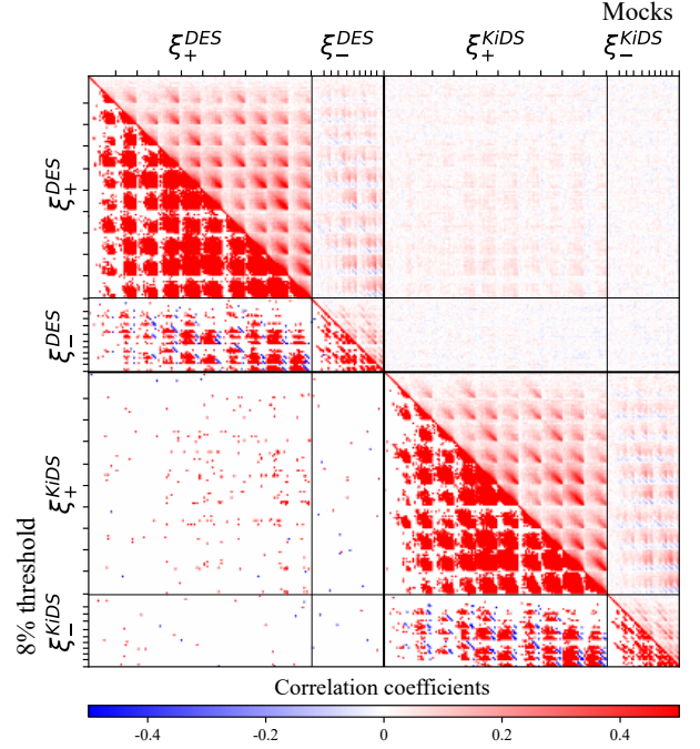
Figure 9. Correlation coefficient matrix for the DES Y3 tomographic cosmic shear data vector measured in two areas: the DES Y3 footprint with the KiDS overlap region excised, denoted \xi_{\pm}(\theta)^{\text{DES}} , and the KiDS-excised region, denoted \xi_{\pm}(\theta)^{\text{KiDS}} . The upper triangle shows the correlation matrix as calculated from FLASK mocks; the lower triangle shows the correlation coefficients above \pm 8\% . The low-levels of correlation between the main DES area and the KiDS-excised area, in the lower-left quadrants, supports our decision to neglect the cross-survey covariance between DES and KiDS in our joint-survey analysis.
