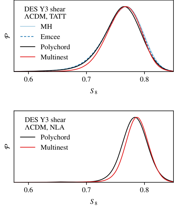
Figure 15. Comparing DES Y3 cosmic shear one-dimensional marginalized posteriors for S_8 obtained using POLYCHORD (black), MULTINEST (red), EMCEE (blue, dashed) and Metropolis-Hastings (MH, light blue) samplers. Results from an analysis using the TATT IA model, matching the posteriors shown in Figure 14, are shown in the upper row, while the lower row adopts an NLA IA model.
