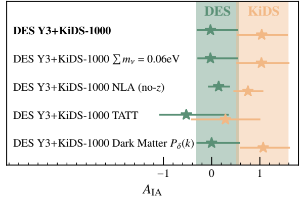
Figure 4. Summary of mean marginalised 1D constraints for the NLA-z A_{\text{IA}} parameter. The top row and shaded bands show the posterior mean and 1\sigma error bars from our fiducial Hybrid pipeline analysis of the joint DES Y3 + KiDS-1000 data vector. In descending order, we show analysis variants with fixed neutrino mass, an NLA analysis with no redshift evolution fixing \eta_{\text{IA}} = 0 , a TATT intrinsic alignment model analysis and an analysis using a dark matter non-linear matter power spectrum with no marginalisation over the effects of baryonic feedback. In the case of the TATT analysis we plot constraints for the a_1 parameter, which is equal to A_{\text{IA}} in the limit where the TATT parameters a_2, \eta_2, b_{\text{TA}} \rightarrow 0 . See Appendix G for marginal constraints on each TATT parameter.
