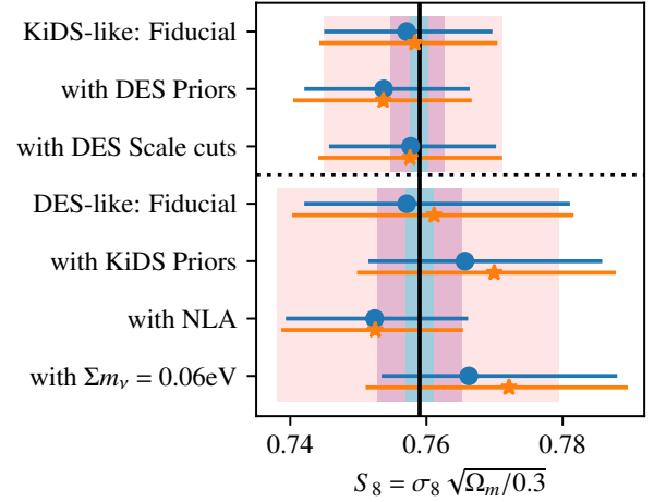
Figure 12. Mock joint-survey S_8 constraints, comparing the KiDS-like (upper section) and DES-like (lower section) fiducial analyses with modifications: adopting an alternative set of cosmological parameter priors (as listed in the second panel of Table 1); adopting alternative astrophysical systematic mitigation strategies with the KiDS-like analysis adopting scale cuts to mitigate baryon feedback (see Appendix B), and the DES-like analysis adopting the NLA model to mitigate IA. We present both the maximum-marginal S_8 and 68% credible intervals (blue circle), and the mean-marginal S_8 and 68% credible intervals (orange star). In this figure the mock data matches each survey’s chosen astrophysical systematic framework, with an identical input cosmology and signal-to-noise. For reference the colour bars show 0.1\sigma , 0.3\sigma and 1\sigma bands from the fiducial analysis, centred on the input S_8 , marked in black. These data are tabulated in Table 8.
