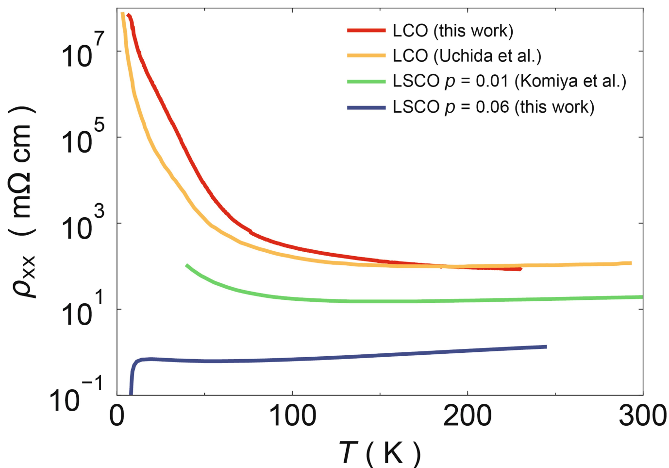
Extended Data Fig. 6 | Electrical resistivity in \text{La}_2\text{CuO}_4 . Electrical resistivity, \rho_{xx} , of two of our samples— \text{La}_2\text{CuO}_4 (LCO, red) and LSCO at p = 0.06 (blue)—compared with published data for \text{La}_2\text{CuO}_4 (yellow 34 ) and LSCO at p = 0.01 (green 35 ). This shows that our LCO sample is very
