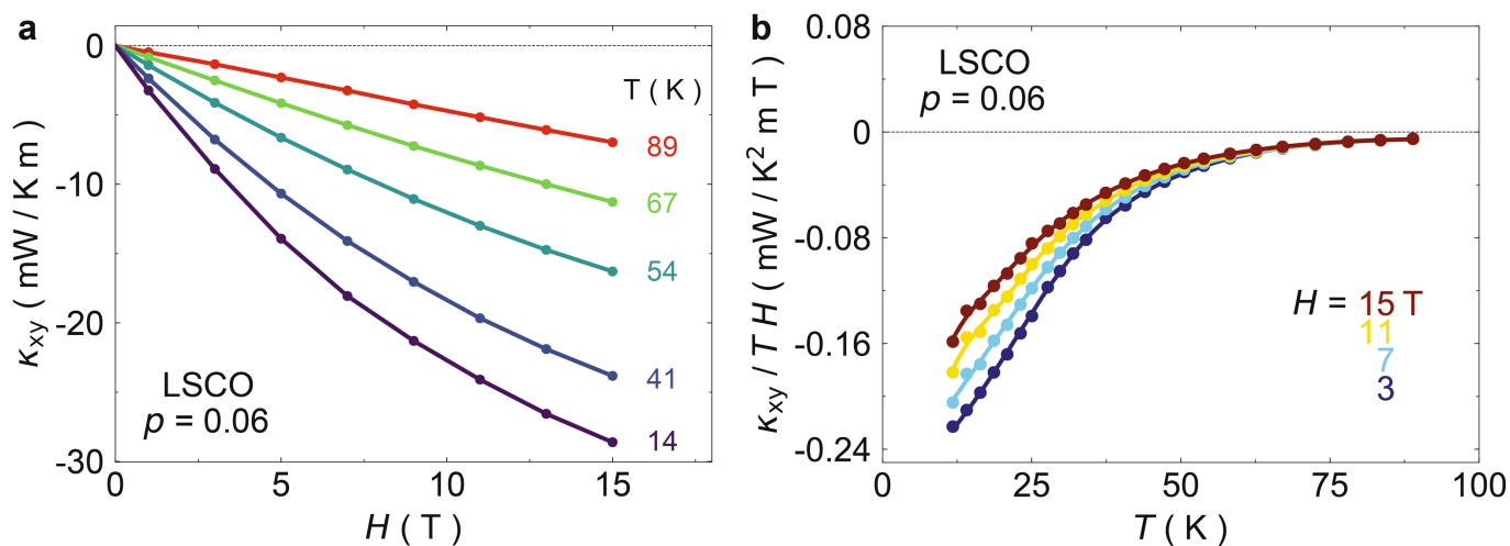
Extended Data Fig. 4 | Magnetic field dependence of \kappa_{xy} in LSCO.
