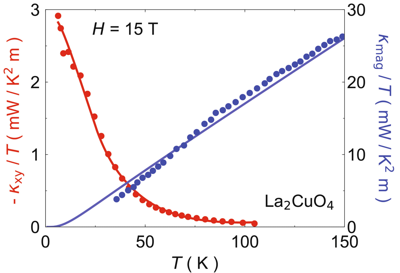
Extended Data Fig. 5 | Magnon thermal conductivity in \text{La}_2\text{CuO}_4 . Thermal conductivity of magnons in \text{La}_2\text{CuO}_4 , plotted as \kappa_{\text{mag}}/T versus T (blue data points, right axis; ref. 37 ). The solid blue line is a fit to the data using the standard calculation for two magnon branches in 2D, with gaps as measured by neutron inelastic scattering 36 , namely \Delta_1 = 26 K and
