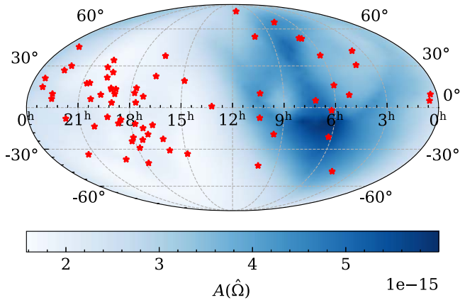
Figure 10. Power measured at each pixel using the Bayesian radiometer pixel basis, in units of characteristic strain, with the red stars showing the position of pulsars in the PTA. This map was constructed with N_{\text{side}} = 8 , resulting in 768 pixels on the sky. Since the prior on the GWB amplitude was log-uniform between 10^{-18} and 10^{-14} , the power was also constrained to be positive across the sky. The sky map is qualitatively consistent with the map derived using the frequentist radiometer pixel basis analysis.
