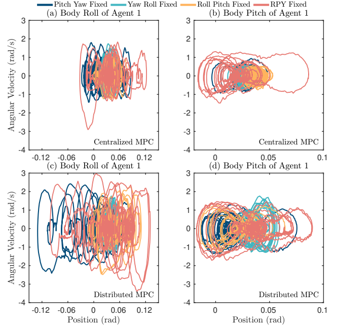
Fig. 25. Phase portraits for (a) the body roll and (b) the body pitch of agent 1 with the centralized MPC and (c) the body roll and (d) the body pitch of agent 1 with the distributed MPC during different experiments. The plots show the robustness of the cooperative locomotion over rough terrain with fixed DOFs in holonomic constraints on the roll, pitch, and yaw directions.
