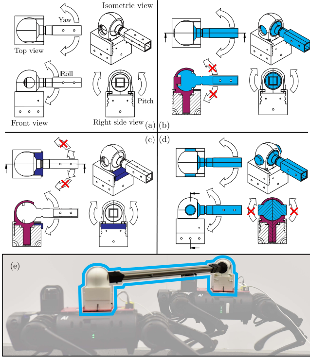
Fig. 5. Illustration of the mechanisms designed to be mounted on the torso of each robot to holonomically constrain the motion of agents. The mechanism in (a) can implement the holonomic constraint in (2) with free ball joints. The mechanisms in (b), (c), and (d) implement the constraint (2) while also restricting the roll, yaw, and pitch motions, respectively. The mechanism implemented on top of the robots is illustrated in (e).
