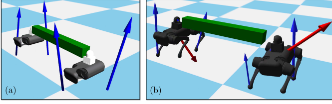
Fig. 7. Snapshots demonstrating the performance of the proposed control approach in numerical simulations. The left figure shows the snapshot of the simulation with the interconnected reduced-order model (torso dynamics) and subject to a 5 (kg) payload (40% uncertainty in one robot's mass) between the agents. The right figure shows the snapshot of the simulation with the full-order model and subject to a 5 (kg) payload between agents and unknown time-varying external disturbances applied to the robots. Arrows at the leg ends describe the GRFs, and the ones on the torso represent the external disturbance forces. The payload is illustrated with a box.
