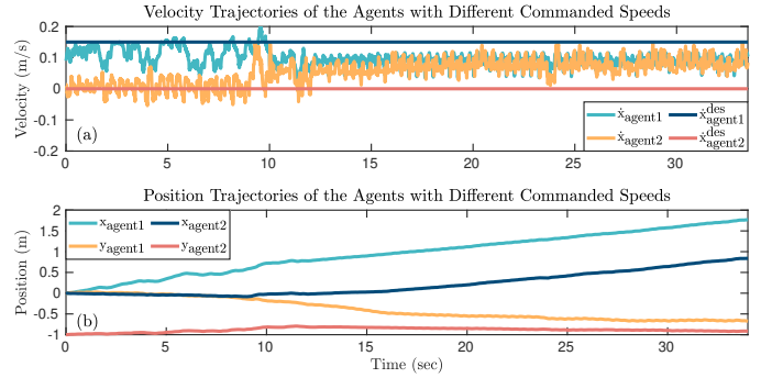
Fig. 9. (a) Plots of the desired and actual velocities of the closed-loop interconnected reduced-order model when the desired velocities are not identical. (b) Plots of the actual COM positions of two agents. The commanded velocity on the first and second agents is taken as 0.15 (m/s) and 0 (m/s), respectively. Here, the optimal GRFs are generated by the distributed MPCs (23).
