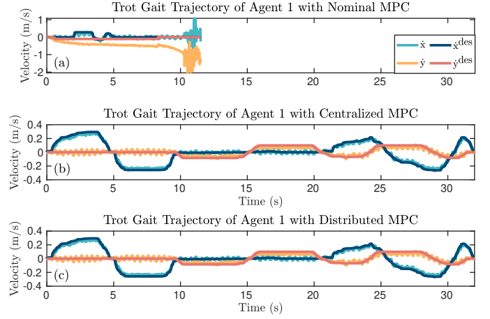
Fig. 8. Plots of the desired and actual velocities of the closed-loop interconnected reduced-order model for two agents in the numerical simulation. Here, the optimal GRFs are generated by the (a) nominal MPCs, (b) centralized MPC (16), and (c) distributed MPCs (23) and are applied to the reduced-order models. An unknown payload of 5 (kg) between agents is applied to the reduced-order models in (b) and (c) to show tracking performance subject to unknown disturbances.
