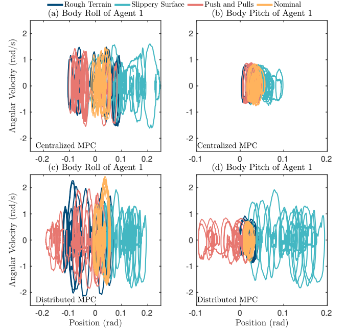
Fig. 16. Phase portraits for (a) the body roll and (b) the body pitch of agent 1 with the centralized MPC and (c) the body roll and (d) the body pitch of agent 1 with the distributed MPCs during different experiments. The plots show the robustness of the cooperative locomotion over rough terrain covered with randomly dispersed wooden blocks, the slippery surface, and subject to unknown external disturbances.
