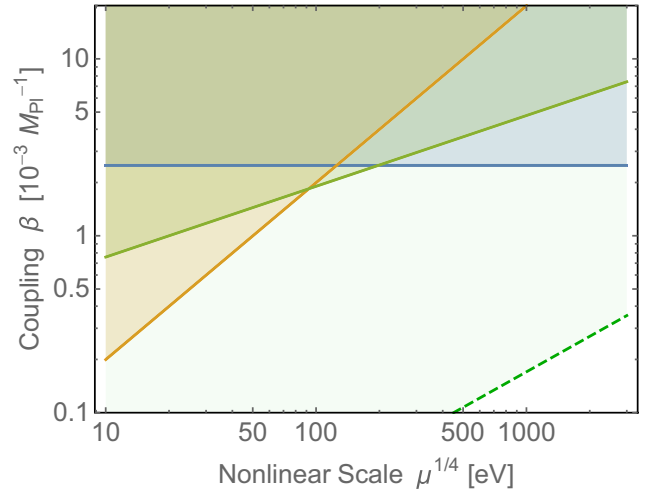
FIG. 2. Observational constraints on the model parameters: Coupling \beta on vertical axis and nonlinear scale \mu^{1/4} on horizontal axis. The blue region is ruled out by solar system tests of light bending. The orange region is ruled out by precession of Hulse-Taylor pulsar binary; this assumes p \sim 5/6 , but it is rather insensitive to its value (assuming p is not extremely close to 1). The green region is ruled out by altering neutron stars significantly and is sensitive to the value of p ; the solid green line is for p = 5/6 , the dashed green line is for p = 3/4 . In general, for lower p the green region becomes larger, for higher p the green region becomes smaller. The remaining lower right region is allowed (depending on p ) according to our analysis here (albeit other phenomena, such as mergers, could affect this).
