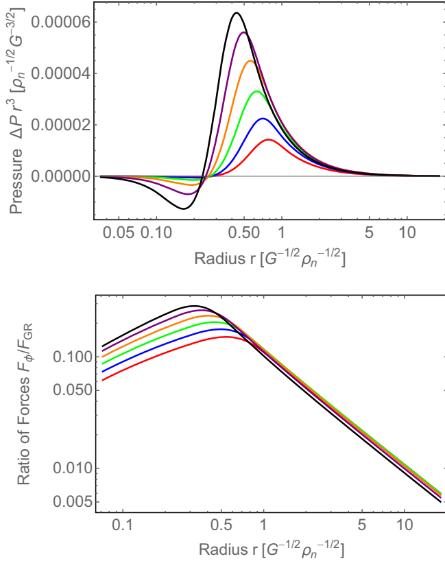
FIG. 6. Top panel: The difference \Delta \mathcal{P} \equiv \mathcal{P}_{\text{eff}} - \mathcal{P} between the effective pressure that sources gravitation and just the neutron pressure; we see that the scalar field creates a considerable amount of positive pressure which explains the extended radius of the star seen in Fig. 4). Bottom panel: The ratio of forces (accelerations) on a unit test mass in a neutron star of the scalar F_\phi = \beta |\nabla \phi| and standard gravity in the Newtonian approximation F_{GR} = Gm(r)/r^2 . The parameters of the model and the color choices are the same as in Fig. 4. Note that outside the neutron star, the ratio is decreasing, since F_\phi \propto 1/r^3 and F_{GR} \propto 1/r^2 . However at very large radii r \gg r_* , the ratio is constant, but that region is not visible here.
