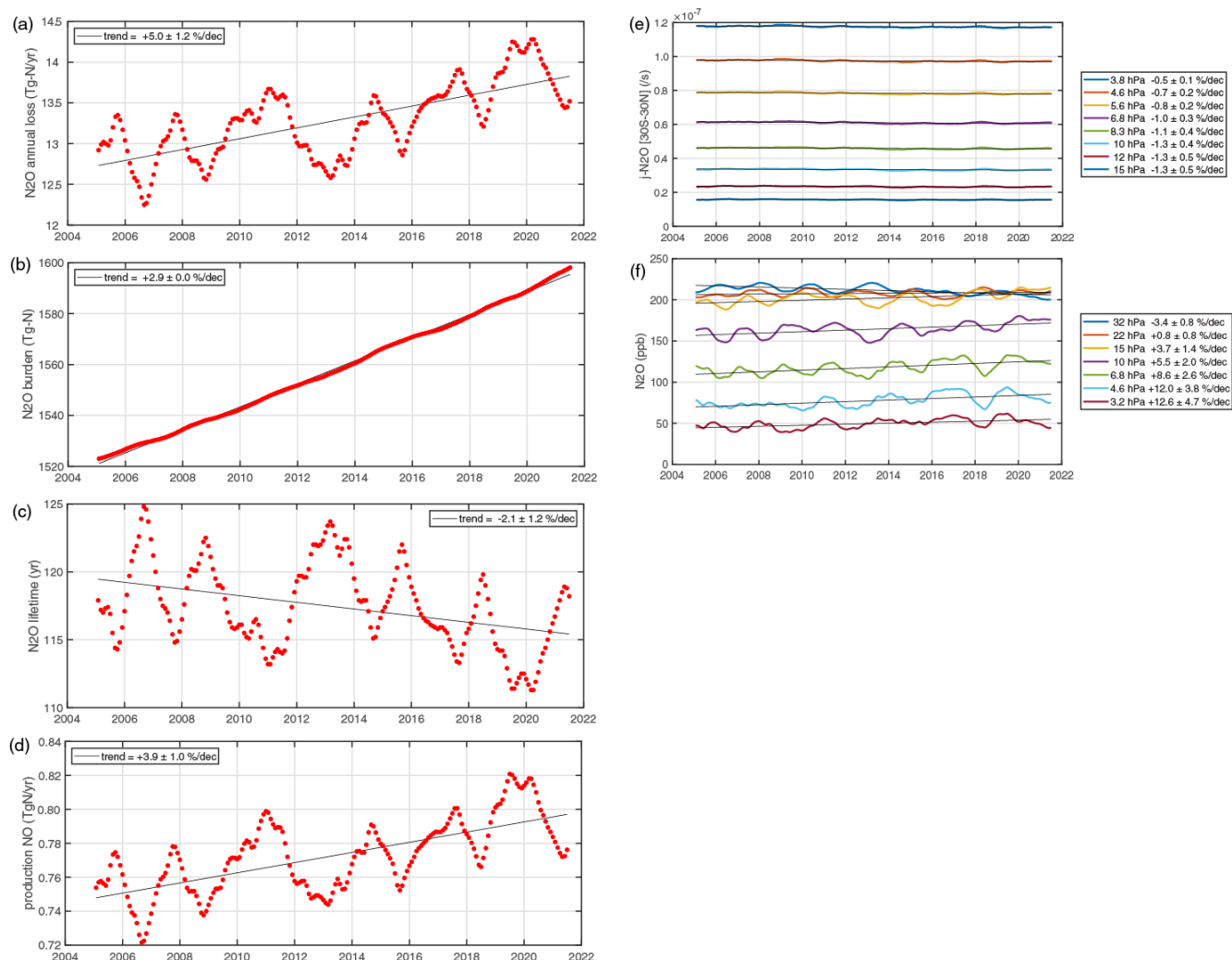
Figure 1. (a) N 2 O loss rate (TgN yr −1 ) as monthly values of a 12-month running mean. The 198 red points begin with the 12-month average of August 2004 through July 2005 plotted as 1 February 2005 with the final point being 1 July 2021 (all of 2021). The thin black trend line shows the slope and uncertainty in the legend; see the text. (b) N 2 O global burden (TgN) based on marine surface observations. (c) N 2 O lifetime derived from the burden divided by loss rate. Production of NO (TgN yr −1 ) from N 2 O loss. (e) Stratospheric photolysis rates, J-N 2 O (/s), at the standard MLS V5 T pressure levels (see legend) and averaged over 30° S–30° N. (f) N 2 O abundance (ppb) at the standard V5 N 2 O pressure levels (see legend) and averaged over 30° S–30° N.
