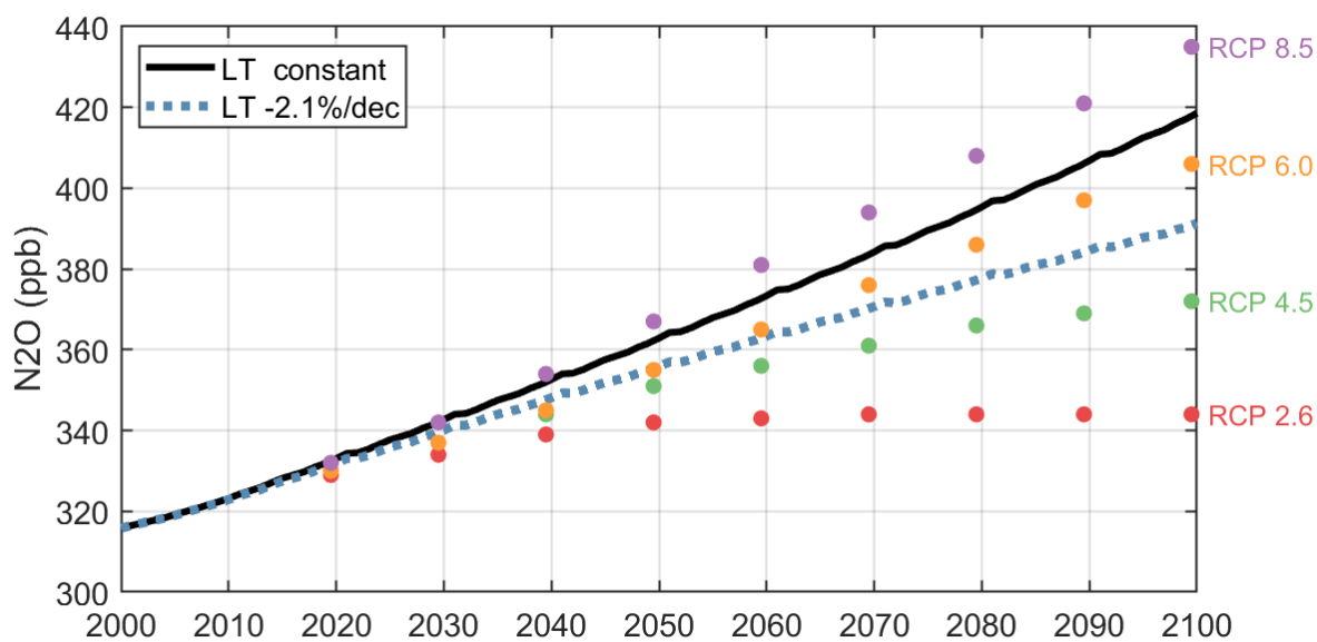
Figure S2. Projected N 2 O tropospheric annual mean abundance (black line) assuming the observed 2.9 %/decade growth rate. The last observed decade 2012-2021 is used to project future decades, and hence there is a recurring interannual variability (IAV). Projected N 2 O with the lifetime decreasing by 2.1 %/decade from 120 y in 2000 to 97 y in 2100 (blue dotted line) uses the emissions inferred from fixed growth scenario. The RCP scenario projections, shown for perspective, are taken from the Annex II tables of the IPCC WGI AR4 (2013).
