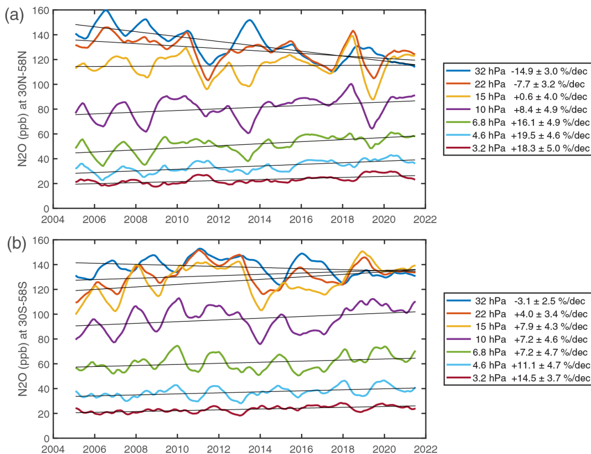
Figure S1. Time series of stratospheric f\text{-N}_2\text{O} (ppb, dry air mole fraction) at (a) northern mid-latitudes (30°N – 58°N) and (b) southern mid-latitudes (30°S – 58°S). See main text Fig. 1
