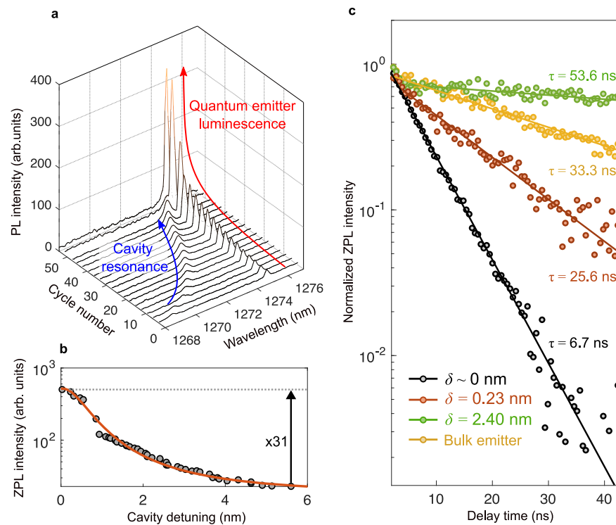
Fig. 4 | Spectral tuning of the nanocavity and enhanced atom-cavity interaction. a The enhancement of the single center in the cavity requires spatial and spectral overlap. Spatial overlap was achieved in Fig. 3 and spectral overlap is achieved here by tuning the nanophotonic cavity. Cavity tuning as a function of the argon gas injection cycle. Gas injection modifies the effective index of cavity mode and tunes the resonance wavelength of the cavity that is shifted from -1269 nm to -1275 nm. As the cavity resonance is shifted towards the ZPL of the quantum center, the photoluminescence is enhanced to reach a maximum at -1275 nm, where the spectral overlap is achieved. b Zero-phonon line intensity as a function of the detuning of the cavity. An enhancement larger than 30 is achieved on resonance. c Excited lifetime for cavity detuning of \delta = 2.40 nm, \delta = 0.23 nm, and \delta = 0.00 nm.
