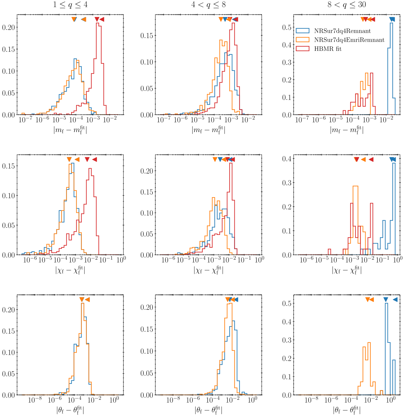
FIG. 3. Test residuals for the extended surrogate (orange) against the previous version of NRSur7dq4Remnant [11] (blue), and the HBMF analytic fits [22,27]. Top, middle, and bottom panels show results for remnant mass m_f/M , spin magnitude \chi_f , and polar angle \theta_f , respectively. Test simulations are divided into three mass ratio bins: NR ( q < 4 , left), near intermediate ( 4 \leq q < 8 , middle), and far intermediate ( 8 \leq q < 30 , right). The left- and down-pointing triangles on top show the 90th percentiles and the median for each of the histograms; the former are also reported in Table I.
