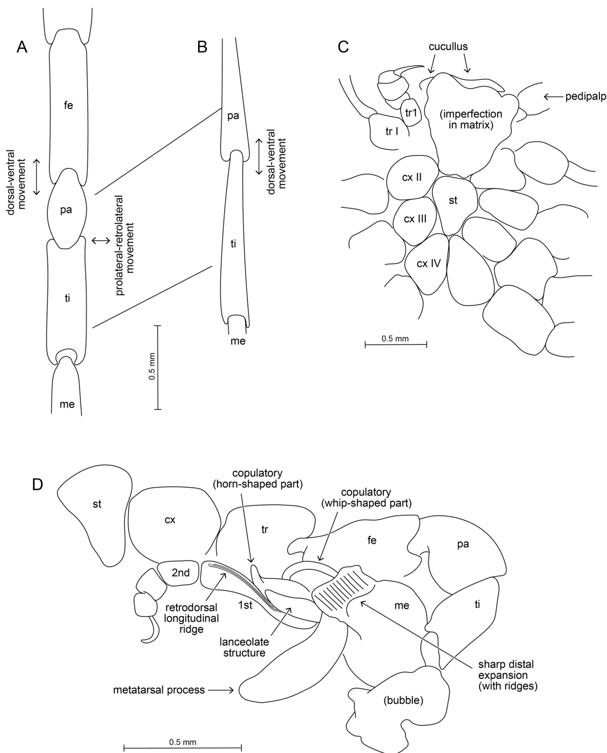
FIGURE 4. Legs and coxosternal region. A and B , Legs, dorsal aspect, of modern ricinuleid (Ricinoididae Ewing, 1929, schematic representation) ( A ) and Hirsutisoma grimaldii sp. nov., holotype ♂ (AMNH_IZC 00357137), dextral leg IV ( B ). C and D , Hirsutisoma grimaldii sp. nov., holotype ♂ (AMNH_IZC 00357137), coxosternal region ( C ) (legs identified by Roman numerals); sinistral leg III, prolateral aspect ( D ) (note modified first tarsomere and unmodified second tarsomere). Abbreviations: cx, coxa; fe, femur; me, metatarsus; pa, patella; st, sternum; ti, tibia; tr, trochanter; tr1, trochanter 1; first and second, proximal tarsomeres.
