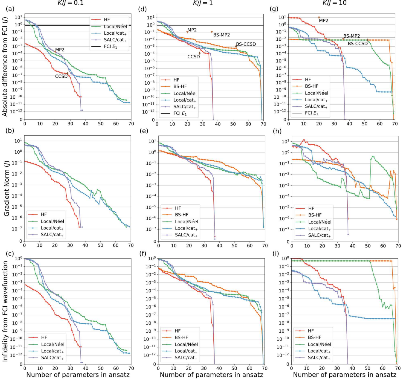
FIG. 3. ADAPT-VQE results for the fermionized, anisotropic Heisenberg Hamiltonian. Absolute energy errors [(a), (d), and (g)], ADAPT-VQE gradient norms [(b), (e), and (h)], and infidelities from the exact wavefunction [(c), (f), and (i)] as the ADAPT-VQE ansätze grow are presented for K/J = 0.1 , K/J = 1 , and K/J = 10 . The ADAPT-VQE methods surveyed use symmetry-preserving HF orbitals and reference state (HF); broken symmetry HF orbitals and reference state (BS-HF); local site orbital basis, Néel reference state (Local, Néel); local site orbital basis, \text{cat}_+ reference state (Local, \text{cat}_+ ); and symmetry-adapted linear combination orbital basis, \text{cat}_+ reference state (SALC, \text{cat}_+ ). Absolute energy errors for the classical methods and the energy gap between the ground and first excited FCI states are presented alongside the ADAPT-VQE errors.
