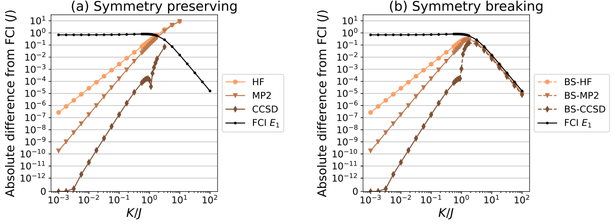
FIG. 2. Absolute energy errors from FCI for HF, MP2, and CCSD versus the correlation parameter K/J presented alongside the energy gap between the ground and first excited FCI states (FCI E_1 ). (a) Reference state is the symmetry preserving orbitals. (b) Reference state is the broken-symmetry orbitals.
