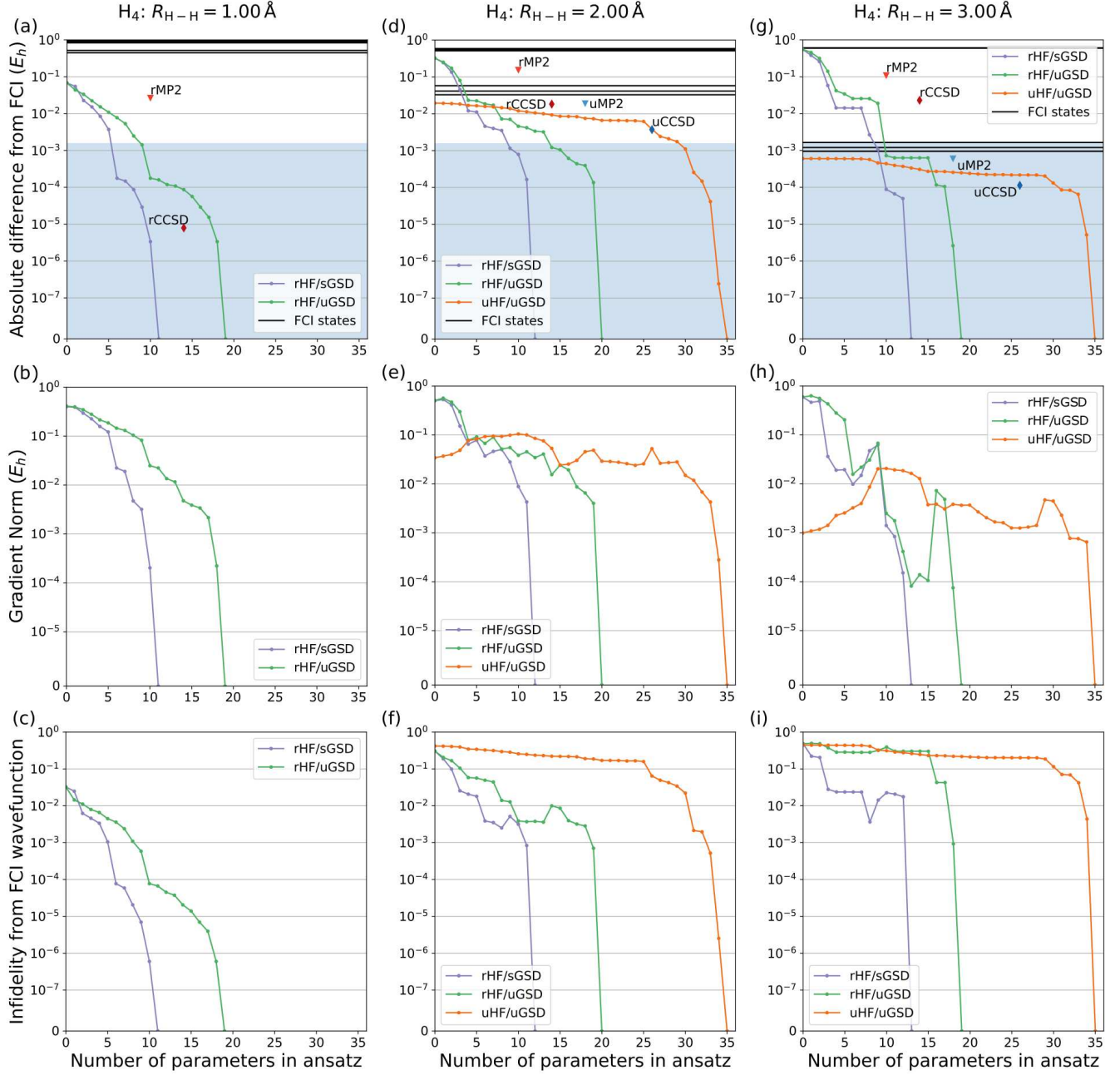
FIG. 5. ADAPT-VQE results for the symmetric dissociation of linear H_4 . Absolute energy errors ((a), (d), and (g)), ADAPT-VQE gradient norms [(b), (e), and (h)], and infidelities relative to the exact wavefunction ((c), (f), and (i)) as the ADAPT-VQE ansätze grow are presented for R_{H-H} = 1.00\text{\AA} , R_{H-H} = 2.00\text{\AA} , and R_{H-H} = 3.00\text{\AA} . The ADAPT-VQE methods with restricted HF orbitals, reference states, and singlet GSD operator pools (rHF/sGSD); restricted HF orbitals, reference states, and unrestricted GSD pools (rHF/uGSD); and unrestricted HF orbitals, reference states, and unrestricted GSD operator pools (uHF/uGSD) are presented. Absolute energy errors for the classical methods and the energy gaps between the ground state and the 9 lowest excited states are presented alongside the ADAPT-VQE errors.
