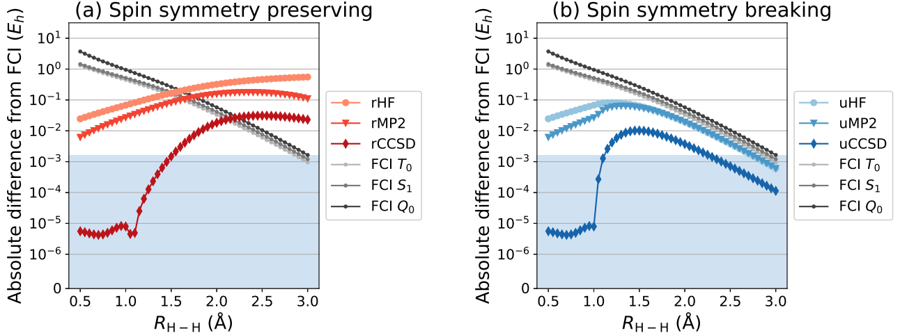
FIG. 4. Absolute energy errors from FCI for HF, MP2, and CCSD versus the H-H separation presented alongside the energy gaps between the ground and next lowest singlet ( S_1 ), triplet ( T_0 ), and quintet ( Q_0 ) excited states. HF spontaneously breaks \hat{S}^2 -symmetry for R_{H-H} > 1.00 Å. The shaded area denotes “chemical accuracy” (errors less than one kcal mol ^{-1} ). (a) Reference state is restricted HF (rHF). (b) Reference state is unrestricted HF (uHF).
