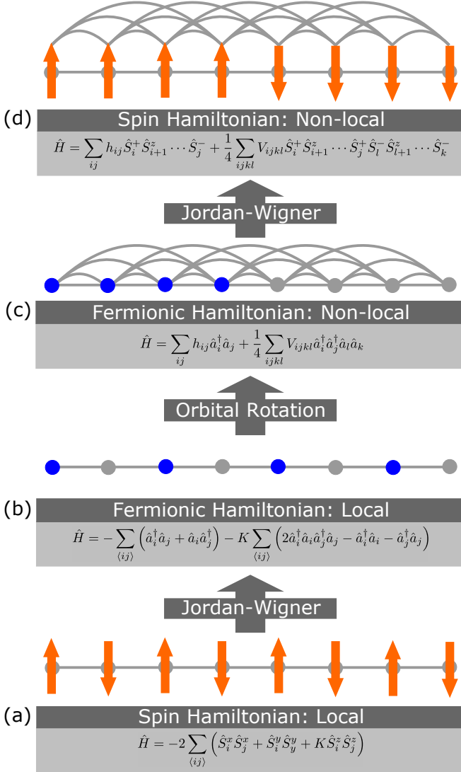
FIG. 1. Depiction of the use of the Jordan-Wigner transformation and Hartree-Fock to transform the anisotropic Heisenberg Hamiltonian from a local representation to a non-local representation. Grey lines between points depict interactions (not all are shown, but meant to represent the locality/non-locality of the system). Constant terms are neglected and J is set to 1.
