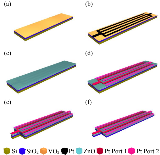
Fig. 5. Step-by-step fabrication process flow of ZnO lateral extensional mode resonators that are equipped with a reconfigurable bottom electrode enabled by the phase transition of the VO 2 thin film.
