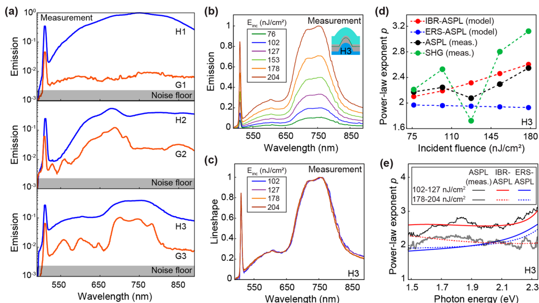
Figure 3. Influence of design geometry and fluence on the upconversion emission spectra. (a) The measured upconversion emission spectra of the H1/G1, H2/G2, and H3/G3 samples under ultrashort pulsed laser excitation (P-polarized, \lambda_{\text{inc}} = 1020 nm, and E_{\text{inc}} = 204 nJ/cm 2 ). H and G samples in each graph share the same TiO 2 capping layer thickness. (b) The measured upconversion emission spectra and (c) lineshapes from the H3 sample under ultrashort pulsed laser excitation (P-polarized, \lambda_{\text{inc}} = 1020 nm) at different fluence levels ( E_{\text{inc}} = 76 nJ/cm 2 up to E_{\text{inc}} = 204 nJ/cm 2 ). (d) The fluence-dependent spectrally integrated power-law exponents ( p ) from the measured SHG (505–515 nm) and ASPL (530–890 nm) signals, and simulations based on the IBR-ASPL and ERS-ASPL models. (e) The spectrally resolved power-law exponents ( p ) from the measured ASPL spectra and simulations based on the IBR-ASPL and ERS-ASPL models at two different fluence ranges.
