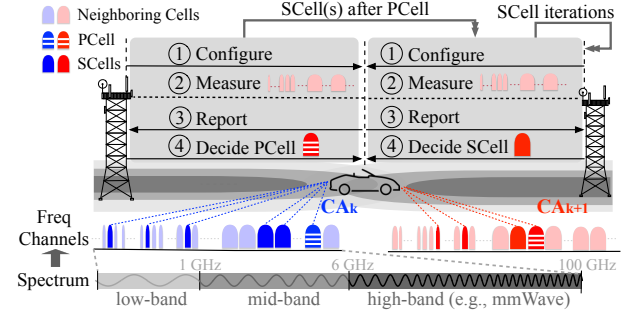
Figure 1: Carrier aggregation under mobility.
