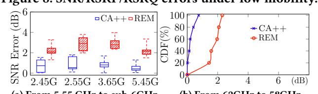
Figure 9: Impacts of measured frequencies.
