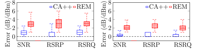
Figure 8: SNR/RSRP/RSRQ errors under low mobility.
