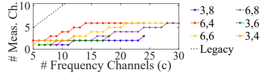
Figure 4: Frequencies to measure (Legend for Q, \bar{k} ).
