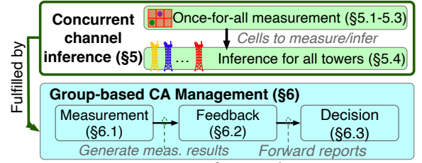
Figure 2: Overview of our solution CA++.
