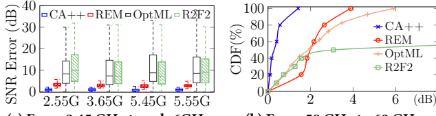
Figure 6: SNR inference errors under low mobility.
