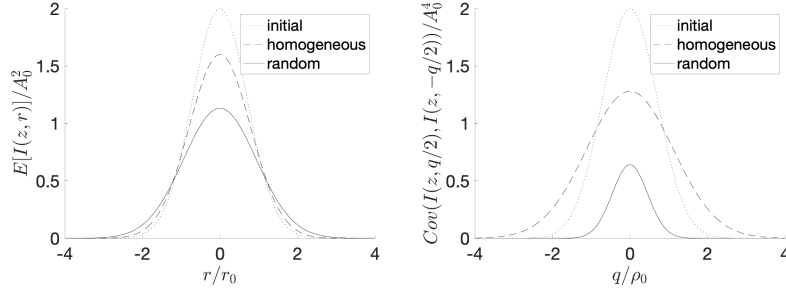
Figure 1. The mean intensity (left) and the intensity covariance (right) when the source is such that \rho_o = 10\lambda_o , r_o = 100\lambda_o (with \lambda_o the wavelength), A_1 = A_2 = A_0 , and \chi = 0 . We compare the profiles of the source (dotted lines) and the profiles of the beam after propagation distance z = z_o/2 in the homogeneous medium (dashed lines) and in the random medium with scattering strength \bar{\gamma}_2 = 5 \cdot 10^{-7} \lambda_o^{-1} (solid lines). Here z_o = k_o \rho_o r_o is the Rayleigh length of the partially coherent source and \bar{\gamma}_2 is defined by Eq. (30) and is a measure of the strength of the random fluctuations in the medium.
