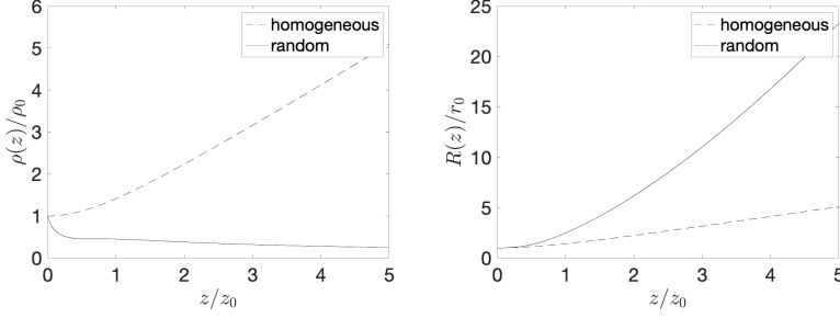
Figure 2. The correlation radius \rho(z) (left) and beam radius R(z) (right) when the source is such that \rho_o = 10\lambda_o , r_o = 100\lambda_o (with \lambda_o the wavelength), A_1 = A_2 = A_o , and \chi = 0 as in Figure 1. We compare the functions in the homogeneous medium and in the random medium with scattering strength \bar{\gamma}_2 = 5 \cdot 10^{-7} \lambda_o^{-1} . Here z_o = k_o r_o \rho_o is the Rayleigh length of the partially coherent source and \bar{\gamma}_2 is defined by Eq. (30).
