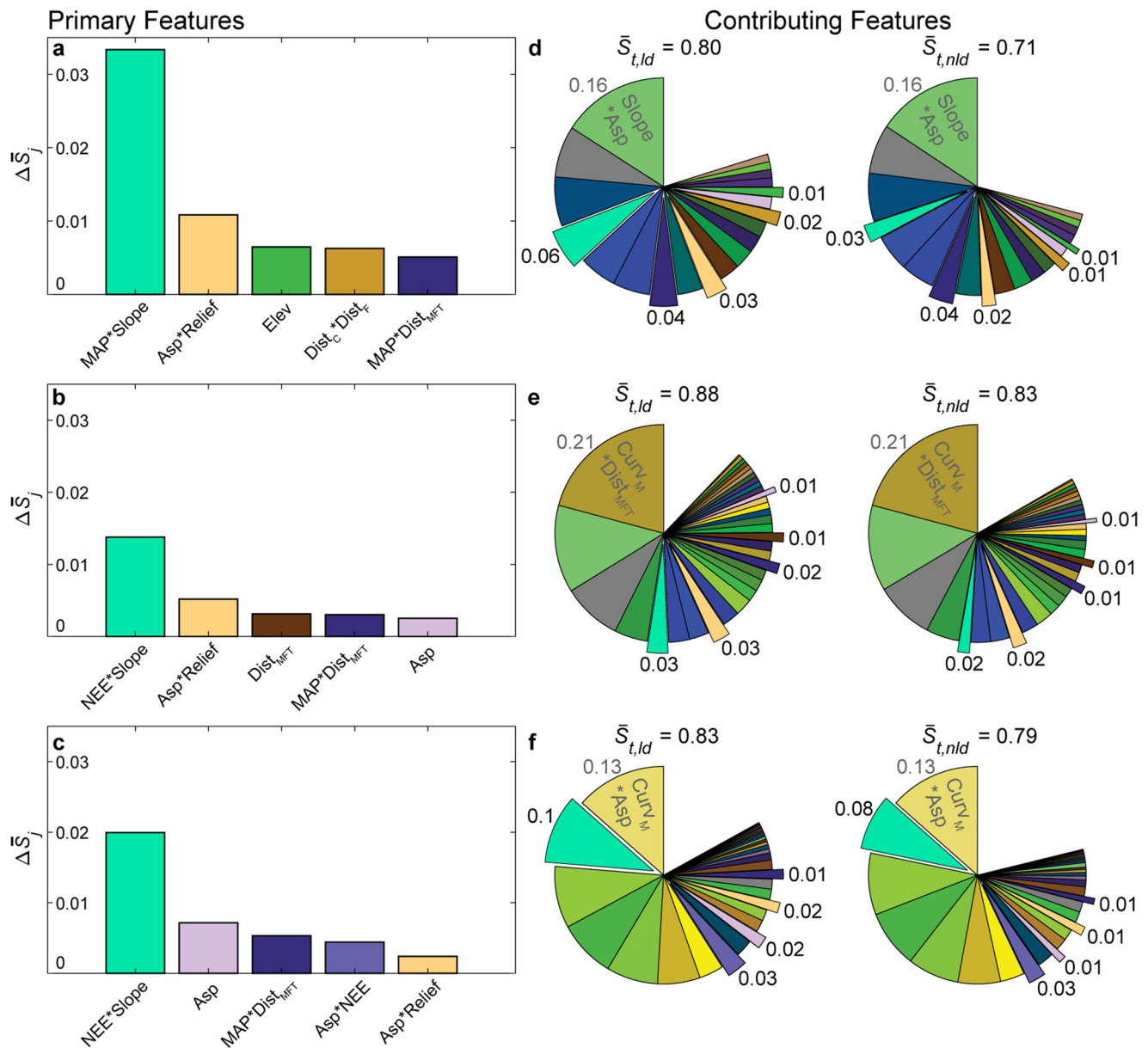
Fig. 7 Feature contributions to total susceptibility. (a, d) N-S, (b, e) NW-SE, and (c, f) E-W study regions. Bar charts in (a–c) represent \Delta \bar{S}_j in descending order, and pie charts in (d–f) represent average S_j ( \bar{S}_j ) contributions to landslide ( ld ) and non-landslide ( nld ) areas. \Delta \bar{S}_j represents the difference in average contribution between areas of ld and nld in each region. Extruding pie chart features are features with large \Delta \bar{S}_j found in the corresponding bar chart on the left. Features related to topography, aspect, climate, and geology are shown in green, pink, blue, and brown or combinations thereof, respectively. Mean annual precipitation (MAP), number of extreme rainfall events (NEE), aspect (Asp), elevation (Elev), mean curvature ( Curv_M ), distances to channel ( Dist_C ), all faults ( Dist_F ), and the Main Frontal Thrust and suture zone ( Dist_{MFT} ), and local relief (Relief). The asterisk * indicates algebraic multiplication of two features. Information regarding features is provided in “Methods”.
