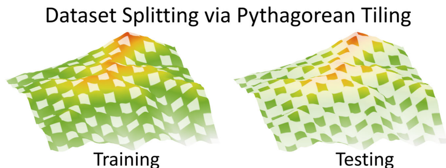
Fig. 5 Illustration of spatial data partitioning using Pythagorean tiling. Pythagorean tiling is used to divide data from the modeled region in a spatially representative manner that maintains variability between training and testing partitions. Using Pythagorean tiling, we generate a checkerboard-like pattern with a 70/30% square ratio, where bigger squares correspond to training and smaller squares correspond to testing.
