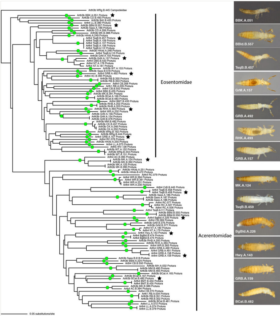
Figure 2. doi Neighbour-joining tree of Appalachian region barcoding sequences, based on K2P distances. Green hexagons on branches indicate ASAP-inferred species level lineages. Black stars indicate specimens pictured at right.
