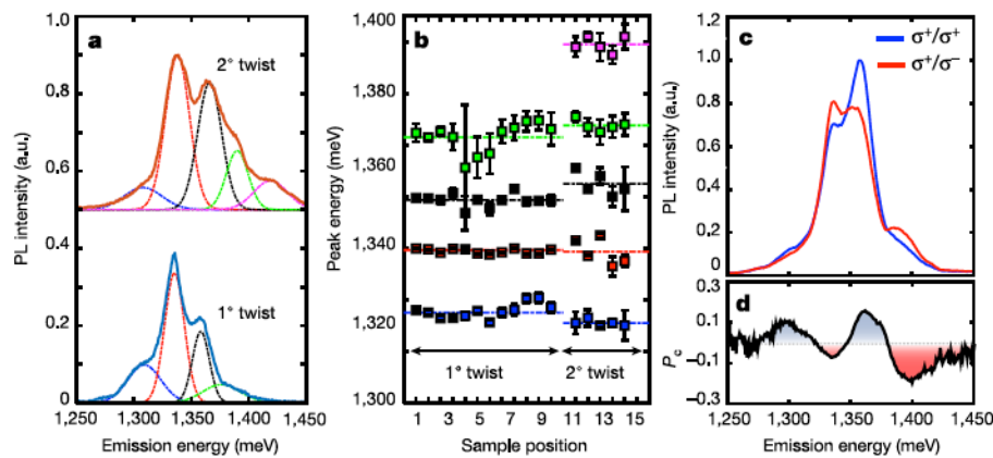
Fig. 3 | Twist-angle dependence and circularly polarized emission. a, Representative photoluminescence spectra shown for heterobilayers with twist angles of 1° (bottom) and 2° (top). Each spectrum is fitted with four (1°) or five (2°) Gaussian functions. b, The centre energy of each peak obtained from the fits at different spatial positions across each sample.
