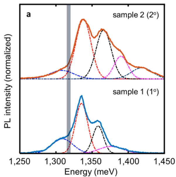
Extended Data Fig. 5 | Comparison of photoluminescence between two heterobilayers with slightly different twist angles. a, Steady-state photoluminescence spectra from the 1° sample (sample 1) and the 2°
