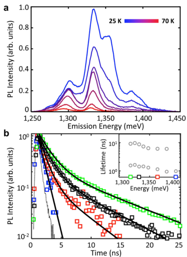
Extended Data Fig. 4 | Thermal decay and recombination dynamics of a heterobilayer with a twist angle of 1°. a, Temperature dependence of the photoluminescence between 25 K and 70 K. b, Time-resolved photoluminescence dynamics (points) at energies close to the four interlayer exciton transitions labelled in the inset. The solid lines are biexponential fits to the data. The inset shows the emission energy dependence of the fast and slow decay times.
