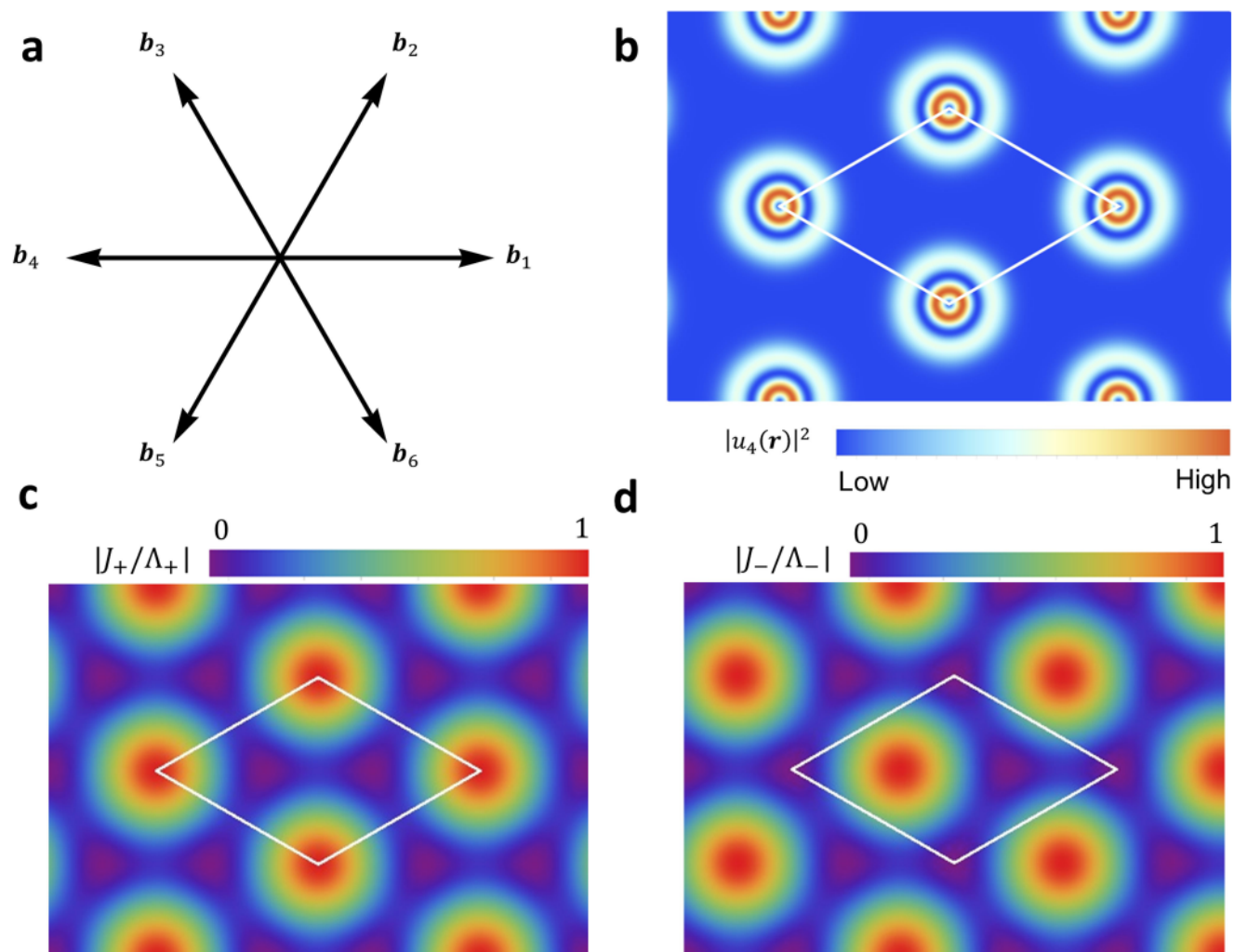
Extended Data Fig. 3 | Moiré exciton theory model. a , Moiré reciprocal lattice vectors in the first shell. b , Real-space map of the centre-of-mass wavefunctions for peak 4. c , d , The spatial variation of the \sigma^+ ( c ) and \sigma^- ( d ) components of the optical matrix elements.
