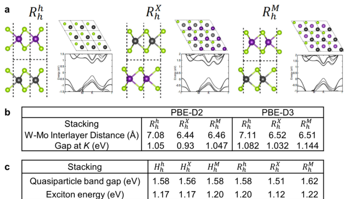
Extended Data Fig. 1 | Band structure. DFT calculation for different stacking types.. a, The three stacking types ( R_h^h , R_h^X and R_h^M ). of the bilayer MoSe 2 /WSe 2 heterostructure and corresponding DFT-calculated band structures. b, Interlayer distance and bandgap of the three stacking types. c, First-principles GW-BSE calculation results for the quasiparticle bandgap and exciton-binding energy of different stacking types.
