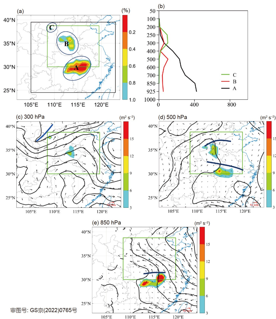
Figure 2 (a) Sensitive areas (shading) identified by the CNOP and (b) the vertical distribution of hTME (units: \text{m}^2 \text{s}^{-2} ) over sensitive area A (black line), B (red line) and C (green line) in panel (a). Wind (vector; units: \text{m s}^{-1} ), Z (contour; units: gpm), and TME (shading; units: \text{m}^2 \text{s}^{-2} ) of CNOP at (c) 300 hPa, (d) 500 hPa, and (e) 850 hPa. The blue line in (c) denotes the trough extending from the cold vortex, and the blue line in (d) and (e) denotes the shear line from the low vortex. The inner green square box in (a), (c), (d), (e) denotes the verification area, and the inner black box in (a) denotes the area for the scale analysis.
