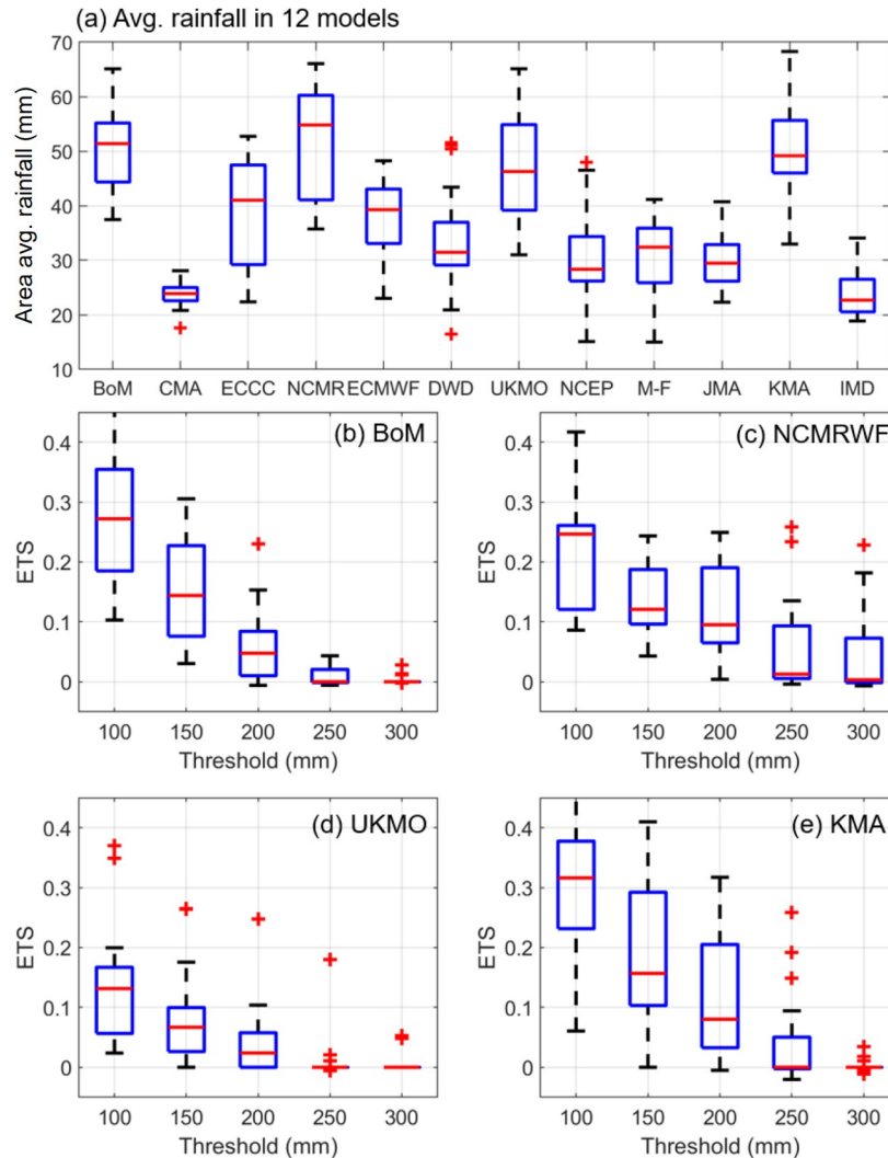
Figure 3 Quantitative precipitation evaluation of ensemble forecasts. (a) Boxplot of area-averaged 24-h accumulated rainfall of ensemble members from the 12 TIGGE models. NCMRWF is denoted by its first four letters (NCMR) owing to the limited space on the x axis. Boxplot of ETSs of ensemble members from (b) BoM, (c) NCMRWF, (d) UKMO, and (e) KMA models at different thresholds from 100 to 300 mm over the focused region. The whiskers extend to the most extreme data points that are not considered outliers. Points are identified as outliers if they are larger than q_3 + 1.5(q_3 - q_1) or smaller than q_1 - 1.5(q_3 - q_1) , where q_1 and q_3 are the 25th and 75th percentiles.
