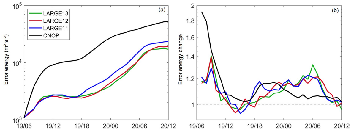
Figure 10 (a) TME (units: \text{m}^2 \text{s}^{-2} ) and (b) hourly growth of the TME over the area interested (the inner black box in Figure 2a) for the CNOP (black line) and LARGE (red, blue and green lines).
