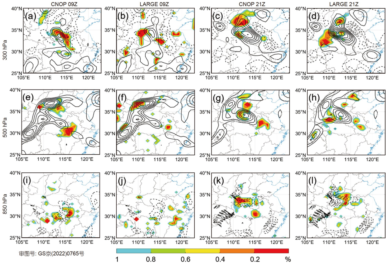
Figure 12 Development of the (first and third columns) CNOP and (second and fourth columns) LARGE_11 at (first and second columns) 0900 UTC and (third and fourth columns) 2100 UTC 19 July 2021. The TME (shading, the top 1% energy) at (upper panels) 300 hPa, (middle panels) 500 hPa, and (bottom panels) 850 hPa. Also shown are (upper panels) the horizontal wind divergence (contour, units: 10^{-5} \text{ s}^{-1} ) at 300 hPa, (middle panels) the vertical relative vorticity (contour, units: 10^{-5} \text{ s}^{-1} ) at 500 hPa, and (bottom panels) the water vapor flux divergence (contour, units: 10^{-4} \text{ kg (kg s}^{-1})^{-1} ) at 850 hPa for the (first and third columns) CNOP and (second and fourth columns) LARGE_11. The solid contour line denotes the divergence area at 300 hPa and positive vorticity at 500 hPa, and the dotted line denotes the convergence area at 850 hPa.
