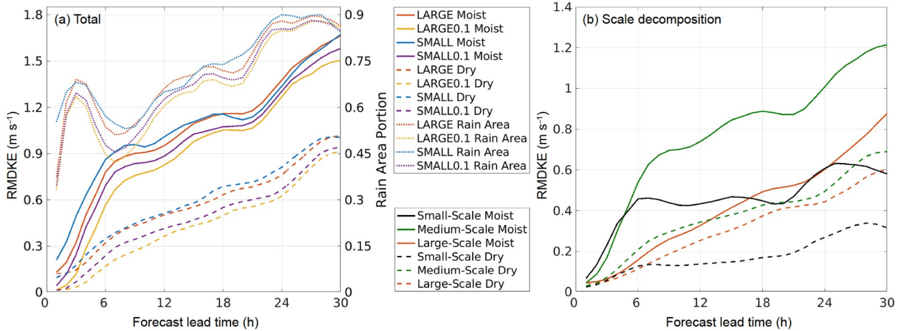
Figure 9 RMDKE of (a) the original model forecast fields, and (b) the model forecast fields decomposed into small scales (<30 km), medium scales (30–200 km), and large scales (>200 km) for regions with (solid lines) and without (dashed lines) precipitation. The portion of the model domain that is covered by precipitation is also plotted in (a) as the dotted lines. The lines in (b) are the averages of respective, scale-decomposed RMDKE values of the four ensembles (i.e., LARGE, LARGE0.1, SMALL, and SMALL0.1).
