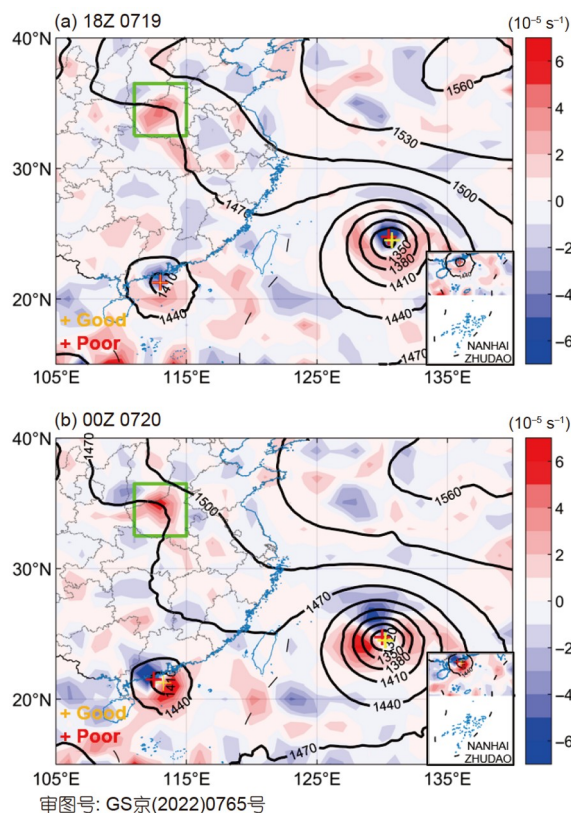
Figure 6 (a) Differences of 850-hPa vertical relative vorticity between composite of good members and poor members (Good – Poor) on 1800 UTC 19 July; ensemble mean 850-hPa Z is contoured in black (in gpm); locations of tropical cyclones (identified based on the minimum of 850-hPa Z) in the composite of good (poor) members were denoted by yellow (red) crosses. (b) is the same as (a) but for 0000 UTC 20 July. The green box indicates the focused region same as the black one in Figure 1.
