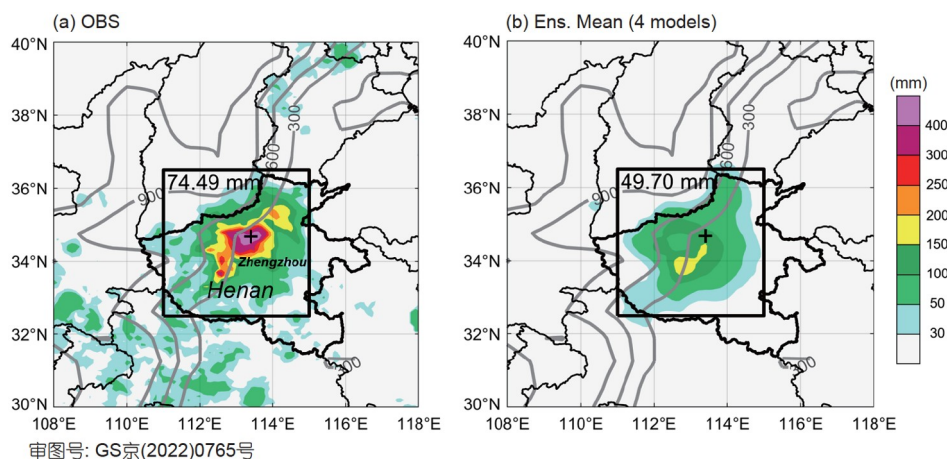
Figure 1 Rainfall distribution in observation and the mean of ensemble forecasts. (a) Observed 24-h accumulated rainfall from 1200 UTC 19 July to 1200 UTC 20 July 2021 (shading; units: mm) and terrain height (grey contour; units: m). (b) Same as (a) but for ensemble mean rainfall forecast initialized at 0000 UTC 19 July based on 4 best-performed models (BoM, NCMRWF, UKMO, and KMA; see text for details). The black box denotes the focused region, and the area-averaged 24-h accumulated rainfall is given on the top left of the box. The location of Zhengzhou City is marked as black cross and Henan Province is outlined in solid black.
