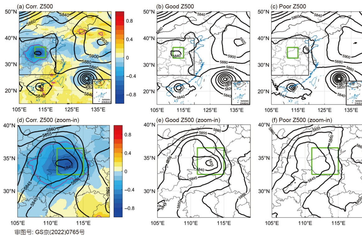
Figure 4 (a) Correlation coefficients (shading; magenta contours for 95% confidence) between the 500-hPa Z at 1800 UTC 19 July and the area-averaged 24-h accumulated rainfall, with ensemble mean 500-hPa Z at respective time contoured in bold black (in gpm); the green box denotes the focused region same as the black one in Figure 1; the grey box denotes the spatial range of (d)–(f). (b) Composite of good members on 500-hPa Z at 1800 UTC 19 July contoured in black (in gpm). (c) is the same as (b) but for composite of poor members. (d)–(f) are the same as (a)–(c) but zoomed in over the grey box given in (a)–(c).
