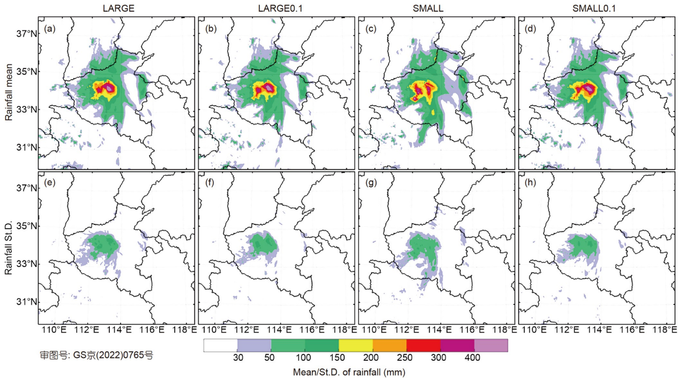
Figure 7 (upper panels) Ensemble probability-matched mean and (lower panels) ensemble standard deviation of 24-hour accumulated rainfall from 1200 UTC 19 July 2021 to 1200 UTC 20 July 2021 for the (first column) LARGE, (second column) LARGE0.1, (third column) SMALL, and (fourth column) SMALL0.1 ensemble forecasts.
