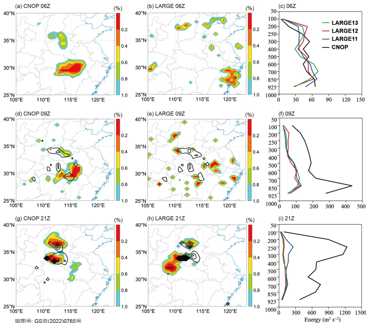
Figure 11 Development of the CNOP and LARGE at (upper panels) 0600 UTC, (middle panels) 0900 UTC, and (bottom panels) 2100 UTC 19 July 2021. The vertical integrated TME (shading, the top 1% energy) for (first column) CNOP and (second column) LARGE 11 , and (third column) the vertical distribution of the hTME (units: \text{m}^2 \text{s}^{-2} ) for CNOP and LARGE are shown. The simulated 1-h precipitation (contour, every 2 mm) at the corresponding time are also shown in (d), (e), (g), (h).
