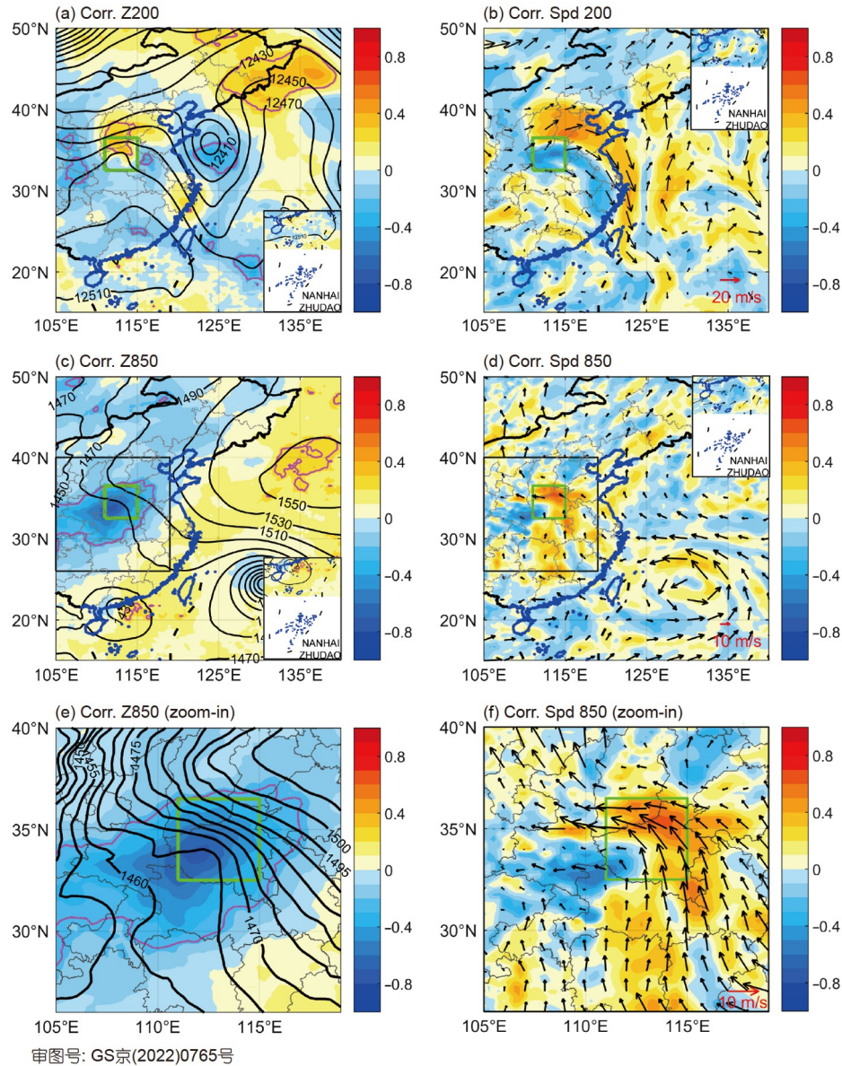
Figure 5 (a) Correlation coefficients (shading; magenta contours for 95% confidence) between the 200-hPa Z at 1800 UTC 19 July and the area-averaged 24-h accumulated rainfall, with ensemble mean 200-hPa Z at respective time contoured in bold black (in gpm). (b) Correlation coefficients (shading) between the 200-hPa horizontal wind speed at 1800 UTC 19 July and the area-averaged 24-h accumulated rainfall, with ensemble mean 200-hPa horizontal wind vector at respective time (reference vector given in bottom right). (c) and (d) are the same as (a) and (b) but for 850 hPa, where the grey box denotes the spatial range of (e) and (f). (e) and (f) are the same as (c) and (d) but zoomed in over the grey box given in (c) and (d).
