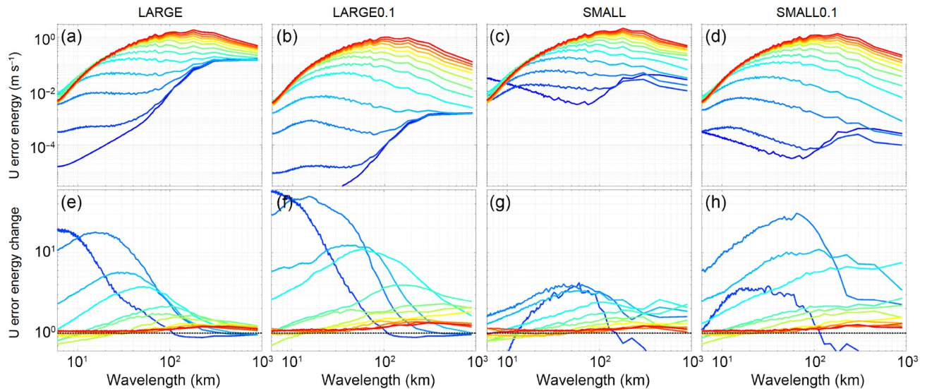
Figure 8 (upper panels) Hourly ensemble-mean power spectra and (lower panels) hourly growth of the ensemble-mean power spectra of the U-wind perturbations from 0600 UTC to 1800 UTC of 19 July 2021 (0 to 12 hours of the ensemble simulation) for the (first column) LARGE, (second column) LARGE0.1, (third column) SMALL, and (fourth column) SMALL0.1 ensemble forecasts. Blue colors denote earlier times (shorter simulation lengths) and red colors denote later times (longer simulation lengths).
