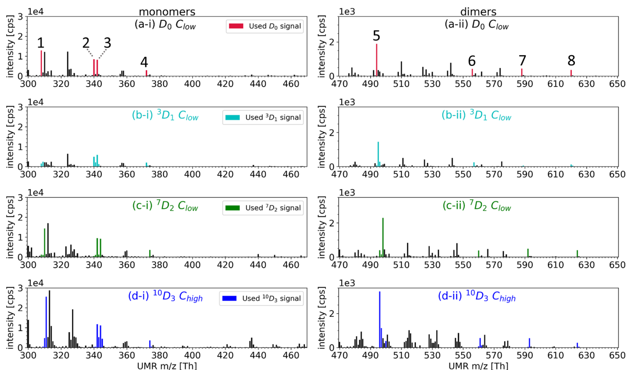
Figure A2. Mass spectra of HOMs from selectively deuterated \alpha -pinene precursors at unit mass resolution. Masses corresponding to HOM signals used on closer inspection are marked with a colour, whereas other peaks in the mass spectra are shown in black. (a-i) and (a-ii) : the closer-inspection compounds are 1. \text{C}_{10}\text{H}_{14}\text{O}_7 , 2. \text{C}_{10}\text{H}_{14}\text{O}_9 , 3. \text{C}_{10}\text{H}_{16}\text{O}_9 , 4. \text{C}_{10}\text{H}_{14}\text{O}_{11} , 5. \text{C}_{19}\text{H}_{28}\text{O}_{11} , 6. \text{C}_{20}\text{H}_{30}\text{O}_{14} , 7. \text{C}_{20}\text{H}_{30}\text{O}_{16} , and 8. \text{C}_{20}\text{H}_{30}\text{O}_{18} . The y scales are different between the monomer and dimer plots.
