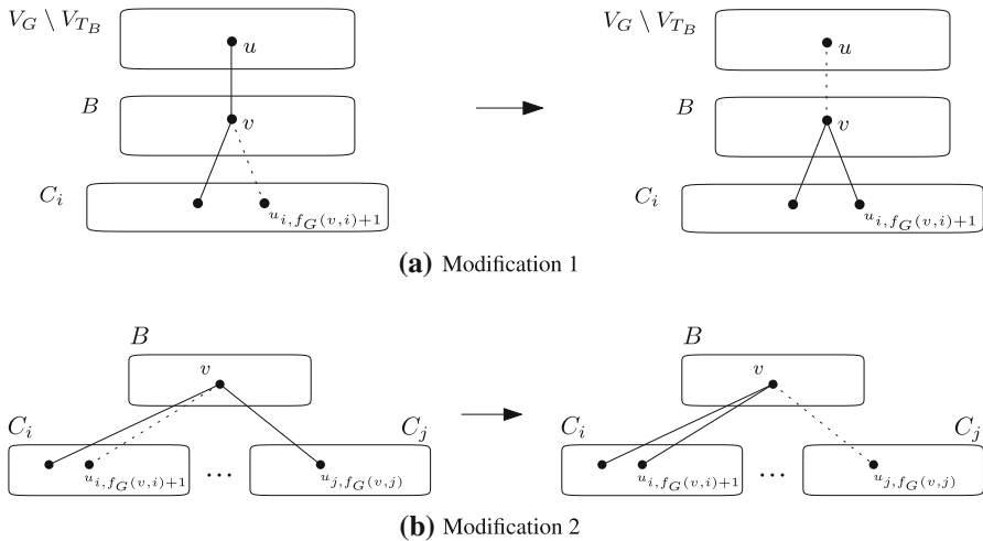
Fig. 1 The dotted lines between two vertices indicate non-edges
