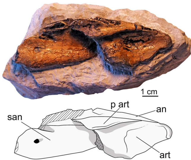
FIGURE 5. Photograph and line interpretation of the posterior region of left mandibular ramus of Turnersuchus hingleyae gen. et sp. nov. (LYMPH 2021/45) exposed in ventral view. Abbreviations: an, angular; art, articular; p art, prearticular; san, surangular.
