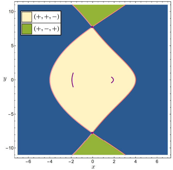
FIG. 1. Parameter space of the matrix H(x, y) in Eq. (9), which obeys H = G^{-1}H^\dagger G where G = \text{diag}(1, 1, -1) . In the blue region of parameter space, pseudo-Hermiticity is broken and the eigenvalues of H are no longer all real. The yellow region is protected from symmetry breaking and has signature (+, +, -) , i.e., the eigenvalue of negative kind is the largest. Similarly, the green region has signature (+, -, +) . Regions of different signatures are topologically disconnected. The boundaries between these regions have exceptional point degeneracies (pink curves), except where the curves meet and annihilate to form a diabolic point (purple points). The central region also contains two disconnected diabolic curves (purple curves) involving two eigenvalues of positive kind. Since they are of the same kind these degeneracies cannot lead to symmetry breaking.
