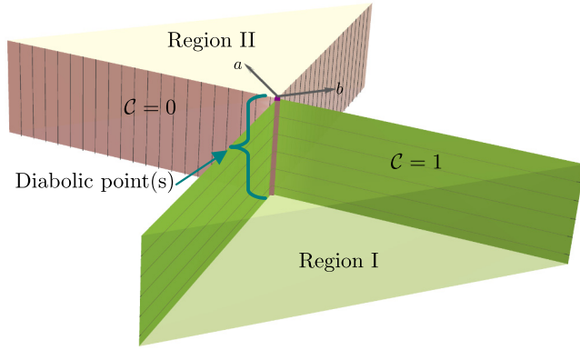
FIG. 2. Strongly stable regions in parameter space (where all eigenvalues are real) are surrounded by exceptional surfaces that meet and annihilate at diabolic points (purple line). These EPs and DPs together make up all possible points where pseudo-Hermiticity breaking occurs. Two such strongly stable regions with signature (\dots, +, -, \dots) and (\dots, -, +, \dots) are shown (labelled I and II respectively). The exceptional surfaces (green with horizontal mesh and pink with vertical mesh respectively) can be identified uniquely with the strongly stable region they enclose and the corresponding signature. Their topological charges can also be written in terms of the zeroth Chern number ( C = 1 and C = 0 respectively). Pseudo-Hermiticity is broken in the region outside these surfaces. In the neighborhood of a symmetry-breaking point, the Hamiltonian can be reduced to the two parameter matrix \begin{pmatrix} a & b \\ -b & -a \end{pmatrix} where a \in \mathbb{R} is a gain-loss parameter and b \in \mathbb{R} is a coupling parameter [see Eq. (11)].
