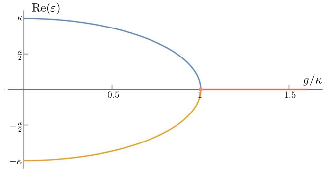
FIG. 3. Real part of the eigenvalues of H = \begin{pmatrix} -ig & \kappa \\ \kappa & +ig \end{pmatrix} , which describes two coupled modes with equal and opposite gain/loss. When g < \kappa , the two eigenvalues, which are of opposite kind, are real. They meet each other at an exceptional point when g/\kappa reaches the threshold value of 1 and on further increasing g/\kappa , the eigenvalues become complex valued.
