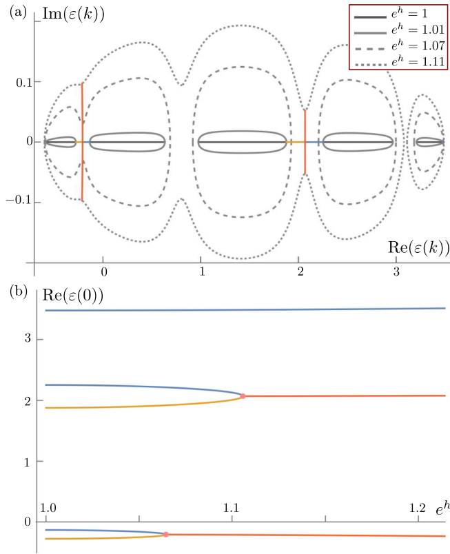
FIG. 5. (a) The eigenvalues of the Hamiltonian in Eq. (21) form M separate oval-shaped bands in the complex plane. Here, we have set M = 5 and V_1 = V_5 = 1.4 , V_2 = V_3 = 1.2 , V_4 = 2 . At h = 0 ( e^h = 1 ), the Hamiltonian is Hermitian and the ovals collapse to line segments on the real axis [dark gray continuous lines in (a)]. As the non-Hermiticity factor h increases, the ovals grow in size and merge with each other (we show the bands at e^h = 1.01, 1.07, 1.11 ). The eigenvalues associated with k \neq 0, \pi move off the real axis at arbitrarily small h while those with k = 0 or k = \pi move along the real axis until a degeneracy of indefinite kind is formed. The trajectories of the eigenvalues of \mathcal{H}(0) [Eq. (24)] on increasing h are depicted by the continuous curves (real eigenvalues of positive and negative kind are shown in blue and yellow respectively, complex-valued eigenvalues are shown in red). These are also shown in (b) where the attraction between eigenvalues of opposite kinds is more apparent. The two symmetry-breaking points shown in pink are both exceptional degeneracies.
