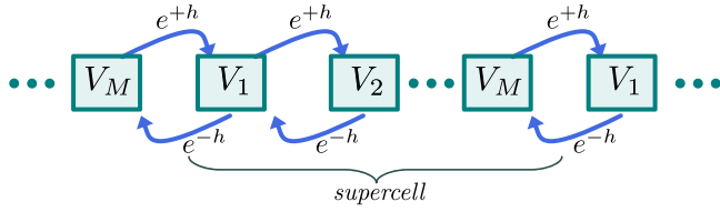
FIG. 4. A lattice with asymmetric hopping described by the Hamiltonian in Eq. (21). Each supercell consists of M sites with on-site potential V_\alpha . The particle hops to the site on its right with amplitude e^{+h} and to the site on its left with amplitude e^{-h} .
