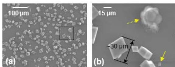
Fig. 7. SEM images of representative calcium carbonate scaling crystals with characteristic lengths of \sim 20 – 50 \mu\text{m} (a) from the region of upstream Raman observation ( x = 5.4 \text{ cm} ). Higher magnification image of the region indicated by the rectangle is shown in (b), where the double arrow depicts an example of a characteristic length measurement. A small calcite crystal with a characteristic length of \sim 5 \mu\text{m} (yellow solid arrow) and a hexagonal-plate vaterite [57] polymorph (yellow dashed arrow) are also observed.
