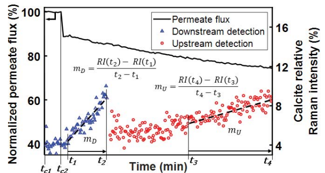
Fig. 3. Representative dataset from a scaling experiment, showing normalized permeate flux and calcite relative Raman intensity over time. The time evolution of the calcite Raman signal is indicated by the dotted lines and calculated for time periods defined by the following timestamps ( t_{\#} ): t_{c1} : Start of membrane compaction phase; t_{c2} : End of membrane compaction phase; t_1 : Start of downstream Raman time evolution; t_2 : End of downstream Raman time evolution; t_3 : Start of upstream Raman time evolution; t_4 : End of Raman upstream time evolution.
