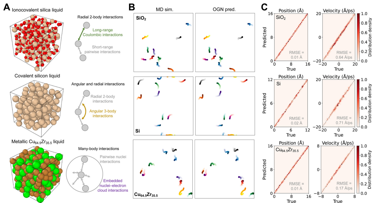
Fig. 3 Simulating complex atom dynamics by OGN. (A) Snapshots of three complex atomistic systems exhibiting distinct types of bonds, including (i) ionocovalent silica (SiO 2 ) liquid governed by radial 2-body interactions, 40 (ii) covalent silicon (Si) liquid governed by both angular and radial interactions, 41 and (iii) metallic Cu 64.5 Zr 35.5 liquid governed by many-body interactions 42 (see text for details). The configuration built for SiO 2 , Si, and Cu 64.5 Zr 35.5 contains 363, 128, and 245 atoms, respectively, and the box side length is set to match their experimental density. (B) True (left panel) versus predicted (right panel) 100-steps atomic trajectories for randomly selected atoms in a test configuration under NVE ensemble for SiO 2 , Si, and Cu 64.5 Zr 35.5 , respectively. The liquids of SiO 2 , Si, and Cu 64.5 Zr 35.5 have been relaxed to an equilibrium temperature around 3600 K, 2000 K, and 1500 K, respectively, and the timestep is set as 1 fs. Note that, due to its low atom diffusivity, we extend the trajectory of Cu 64.5 Zr 35.5 to 400 steps for visibility. (C) Density scatter plot of the predicted versus true atom positions (left panel) and velocities (right panel) (along x -, y -, and z -axis) in the test configuration at the last step for SiO 2 , Si, and Cu 64.5 Zr 35.5 , respectively. The y = x line (grey dash) is added as a reference.
