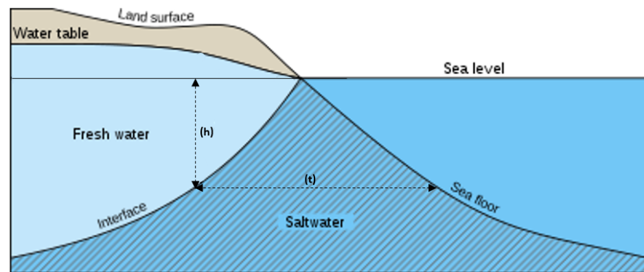
Figure 3. A diagram of a coastal aquifer showing the main seawater intrusion (SWI) metrics.
