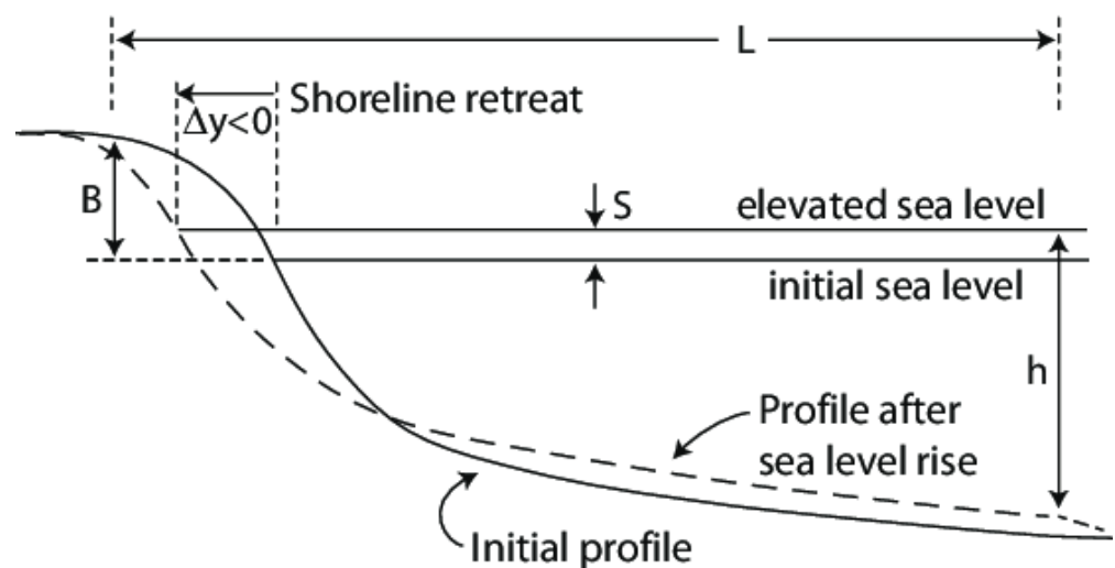
Figure 2. Bruun Rule of shoreline retreat.
