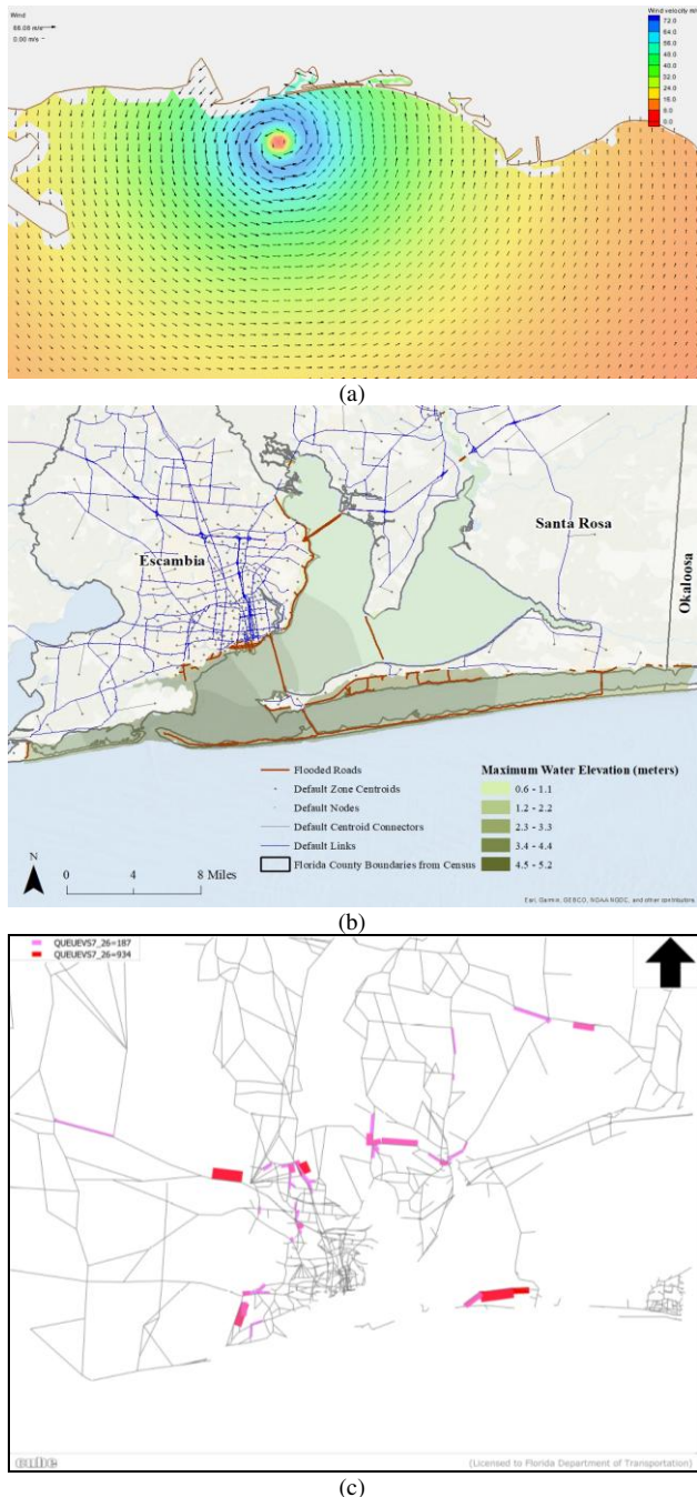
Figure 5. Hurricane Impact Simulation of Pensacola Area – Counties: Escambia, Santa Rosa. (a) Storm Surge with Wind Field Results, (b) Integration of Inundation Results and Transportation Network, and (c) Congested Roads of Pensacola Scenario.
