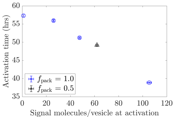
FIG. 10. Activation time in a 2000-cell colony vs average number of signal molecules per vesicle at the time of colony activation. The blue data points correspond to scenarios with one molecule per vesicle, to scenarios with the signal molecules being split evenly among four vesicles at vesicle generation events, to scenarios with the signal molecules being split evenly among two vesicles at vesicle-generation events, and to the scenario considered in the main text (left to right). The black data point corresponds to the scenario f_{\text{pack}} = 0.5 in Fig. 8. All data points and error bars were calculated from ten simulation replicates.
