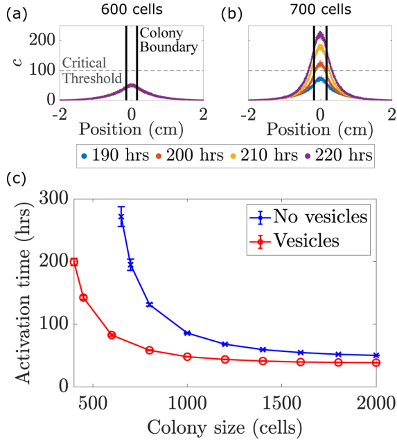
FIG. 2. Vesicle-assisted transport of QS signal molecules reduces the critical colony size required for colony activation and accelerates the activation dynamics. Time progression of the distribution of freely diffusing signal molecules for a system with no vesicle production with (a) 600 cells and (b) 700 cells. Vertical lines indicate colony boundaries and horizontal dashed lines indicate the critical concentration of signal molecules required for activation, c_{\text{crit}} = 100 . The distributions shown are averages over ten simulation replicates, and the vertical axes are identical in both panels. (c) Time to complete colony activation vs colony size for simulations of single colonies with and without vesicle transport of signal molecules. Data points and error bars represent the average activation time and standard deviation from ten simulation replicates.
