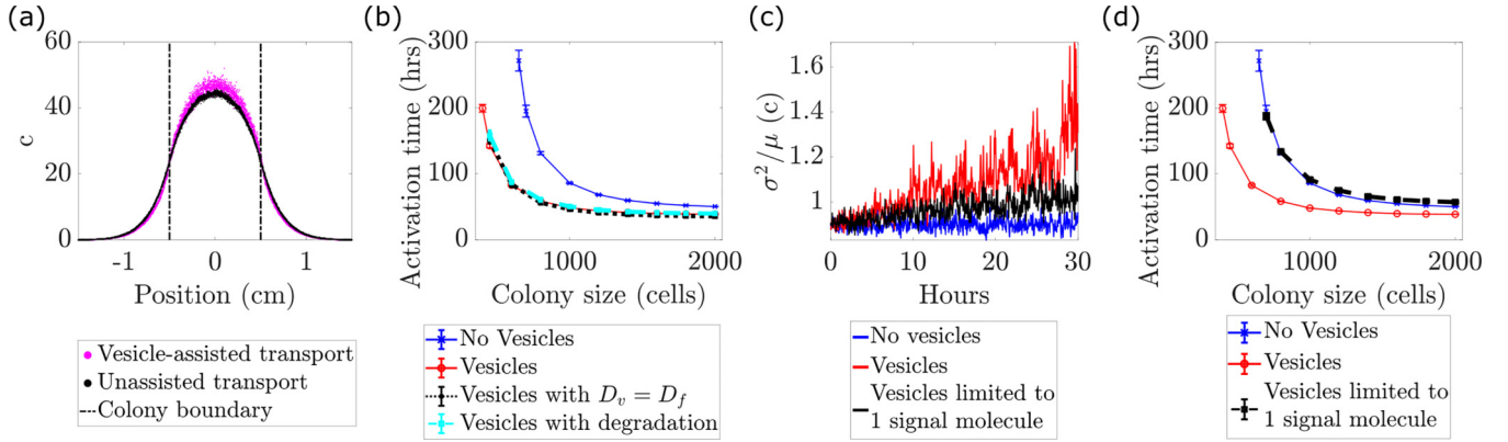
FIG. 3. Physical origins of improved signal transfer through vesicles. (a) Distribution of all QS signal molecules in a system of 2000 cells producing (magenta) or not producing (black) vesicles. Both distributions are shown at the same time point of 25 h. (b) Colony activation time vs colony size for simulations with D_v = D_f (black dashed curve) and the same degradation rate \gamma for signal molecules packaged inside vesicles and freely diffusing signal molecules (cyan dashed curve), compared to the corresponding activation curves with and without vesicles in Fig. 2(c). (c) Fano factor for the signal concentration vs time for a cell at the center of a 2000 cell colony. The data shown here were obtained from a moving average with a 0.1-h time window. (d) Colony activation time vs colony size for cells producing vesicles with only one QS signal molecule per vesicle, compared to the corresponding activation curves with and without vesicles in Fig. 2(c) (see Appendix B for intermediate numbers of signal molecules packaged per vesicle). All results in this figure were obtained by averaging over ten simulation replicates with error bars representing standard deviations. Unless indicated otherwise, we used the same parameter values as in Fig. 2(c).
