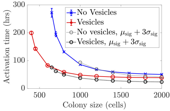
FIG. 7. Estimated colony activation time vs colony size without (gray) and with vesicles (black) as in Eq. (A8) but with a fluctuation envelope corresponding to \mu_{\text{sig}} + 3\sigma_{\text{sig}} and QS signal-molecule concentrations estimated from simulations without vesicles and without allowing cells to activate. The blue and red curves are identical to the corresponding results in Figs. 2 and 3 and reproduced here for ease of comparison.
