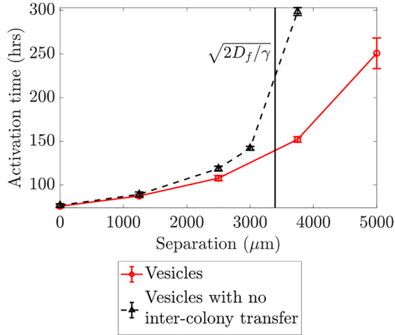
FIG. 6. Intercolony vesicle exchange can strongly affect colony activation for fast enough degradation of free signal molecules and rapid vesicle diffusion. Time to complete activation of a 100-cell colony vs edge-to-edge separation from a neighboring 2000-cell colony. Free signal decay is increased here such that \gamma = 0.05 \text{ h}^{-1} and the vesicle-diffusion coefficient is increased such that D_v = D_f = 80 \mu\text{m}^2 \text{ s}^{-1} , resulting in the characteristic length scale \sqrt{2D_f/\gamma} \approx 3400 \mu\text{m} . Similarly as in Fig. 5, the curves shown compare scenarios in which vesicles can (red curve) and cannot (black curve) contribute to signal exchange between colonies.
