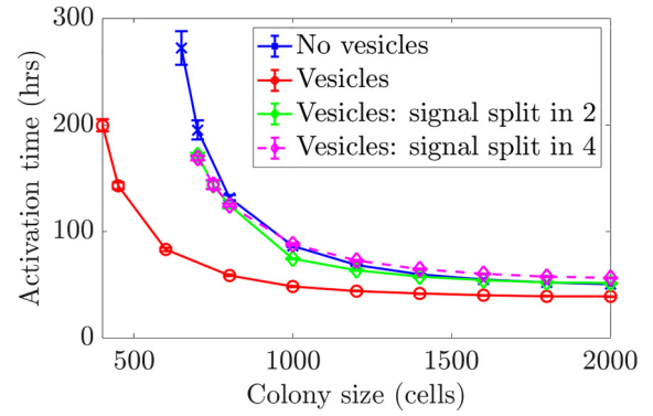
FIG. 9. Colony activation time vs. colony size obtained with no vesicles, with the algorithm for vesicle generation employed in the main text, and with the signal molecules being split evenly between two or four vesicles at vesicle-generation events. Splitting signal molecules among multiple vesicles at vesicle-generation events reduces the number of signal molecules per vesicle, and increases the activation time. All data points and error bars were calculated from ten simulation replicates.
