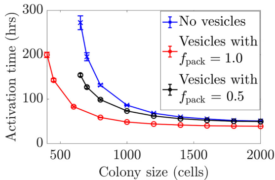
FIG. 8. Colony activation time vs. colony size obtained with no vesicles, vesicles with f_{\text{pack}} = 1.0 , and vesicles with f_{\text{pack}} = 0.5 . Reducing the fraction of signal molecules packaged into vesicles weakens the overall effect of vesicles on the colony activation dynamics. The data points and error bars were calculated from ten simulation replicates.
