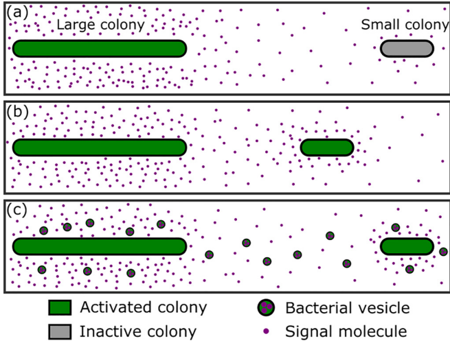
FIG. 4. Large colonies can activate smaller colonies that are otherwise unable to activate. (a) For large enough colony separations, the larger colony does not activate the smaller colony over a given timescale, while (b) over the same timescale activation of the smaller colony by the larger colony may be achieved at smaller separations. (c) Bacterial vesicle production can result in more rapid activation of the smaller colony by the larger colony, and yield intercolony activation over larger colony separations.
