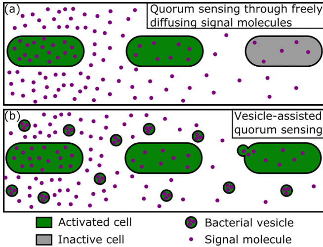
FIG. 1. Bacterial cells utilize two distinct pathways for the transport of QS signals. (a) In the classical model of QS, bacterial communication is mediated exclusively by freely diffusing signal molecules. (b) According to a newly emerging picture of cellular communication, cells utilize both freely diffusing signal molecules and signal molecules packaged in bacterial vesicles to facilitate QS.
