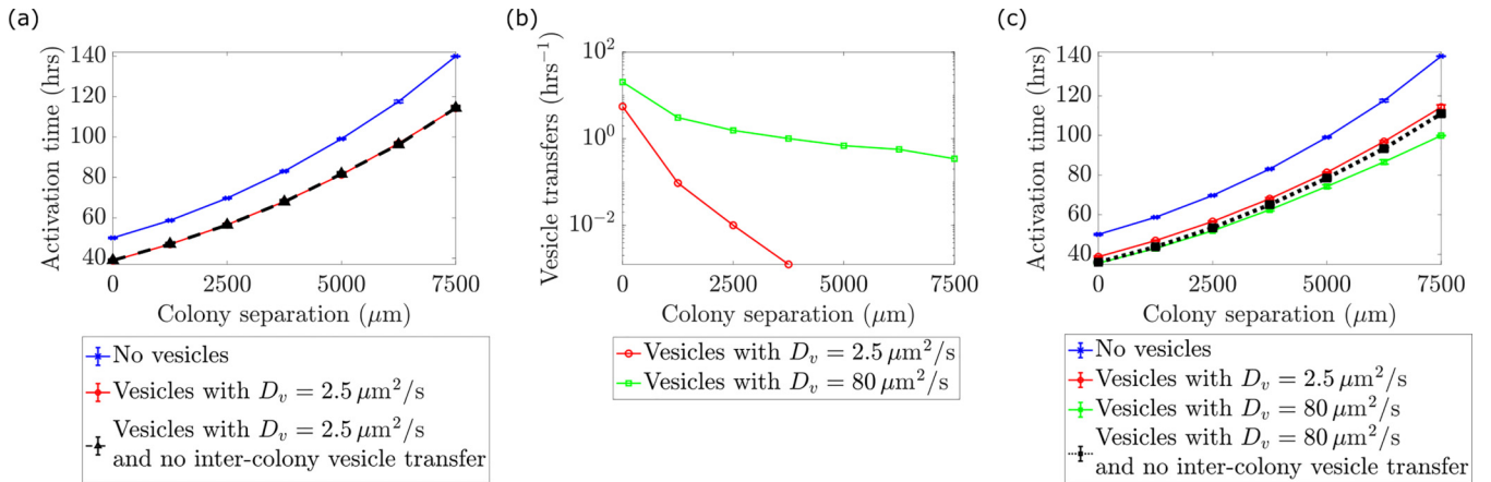
FIG. 5. Vesicle-assisted signal transport in a two-colony system. (a) Time to complete activation of a 100-cell colony vs edge-to-edge separation from a neighboring 2000-cell colony, for bacteria producing no vesicles (blue curve), bacteria producing vesicles (red curve), and bacteria producing vesicles with no intercolony vesicle transfer (black dashed curve). (b) Average rate of vesicle transfer from the larger colony to the smaller colony from t = 0 to complete activation of the smaller colony vs colony separation for the reference value of the vesicle-diffusion coefficient used here, D_v = 2.5 \mu\text{m}^2/\text{s} (red curve), and an increased vesicle-diffusion coefficient, D_v = D_f = 80 \mu\text{m}^2/\text{s} (green curve). (c) Time to complete activation of the smaller vs colony separation as in panel (a), with the increased diffusion coefficient D_v = D_f = 80 \mu\text{m}^2/\text{s} (green curve) and D_v = D_f = 80 \mu\text{m}^2/\text{s} but no intercolony vesicle transfer (black dashed curve). We used the same colony sizes for all panels. The data points show averages and the error bars indicate the corresponding standard deviations from ten simulation replicates each.
