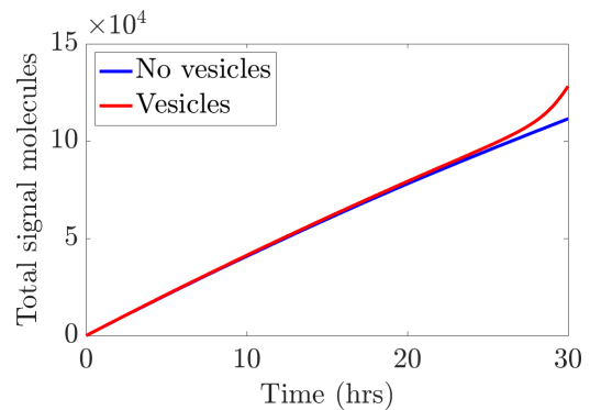
FIG. 11. Total number of signal molecules in the system as a function of time for a colony of 2000 cells, with and without vesicles. We used the same parameter values as in Fig. 3(a). Both curves were obtained by averaging over ten simulation replicates.
