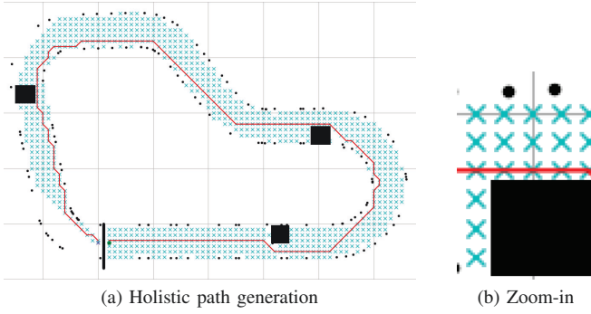
Fig. 2. A-Star path generation.
