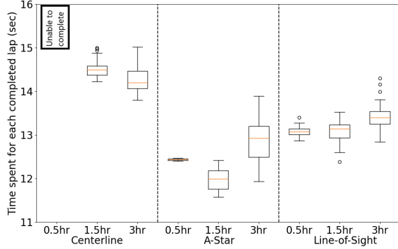
Fig. 5. Time spent on completed laps to show the racing speed of models.
