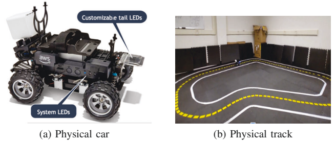
Fig. 1. Physical environment.
