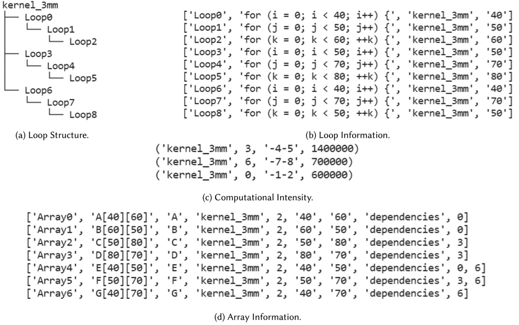
Fig. 7. An example of the information gathered by the Lexical Analyzer.
