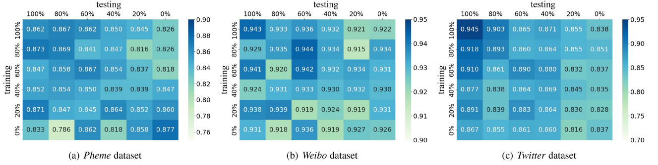
Fig. 4. Classification accuracy on PHEME, Weibo and Twitter datasets with different missing patterns. The row (resp. column) of the matrix represents the percentage of the training (resp. testing) instances that are equipped with the visual data. The darker the blue, the higher the accuracy.
