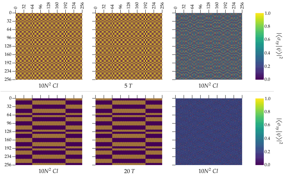
Figure 1: Color map representation of a 16-qubit state after 10N^2 random Clifford gates, then n_T random T gates (Top row: n_T=5 . Bottom row: n_T=20 ), then another 10N^2 random Clifford gates are applied, starting with the initial state |\psi_0\rangle = |0\rangle^{\otimes N} . The image is arranged by partitioning the state into two equal subsystems and expanding one along each axis. A pixel at some position (x, y) is mapped from the magnitude of the amplitude for the computational basis state |\sigma_{xy}\rangle = |\sigma_x\rangle \otimes |\sigma_y\rangle (for example, the pixel at (0, 0) corresponds to the state |\sigma_{00}\rangle = |0\rangle^{\otimes N/2} \otimes |0\rangle^{\otimes N/2} ). The action of a T gate, being a phase gate, does not change the color map representation at all. However, after being spread around by the second Clifford circuit, the color map representation becomes more mixed for the circuit with the larger number of inserted T gates, showing the interplay between the non-Clifford resources and the operator spreading through Clifford-driven entanglement in the onset of quantum chaos.
