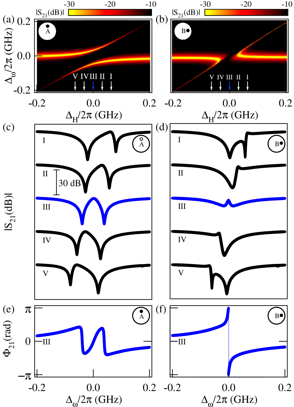
Fig. 13. Observation of magnon–photon level repulsion and level attraction by setting a YIG sphere in the 1D waveguide depicted in Table 1. (a) and (b) are the measured dispersions, while (c)–(f) are the measured amplitude and the phase of the transmission coefficient. Source: Adapted from Harder et al. [161]. Copyright by the American Physical Society.
