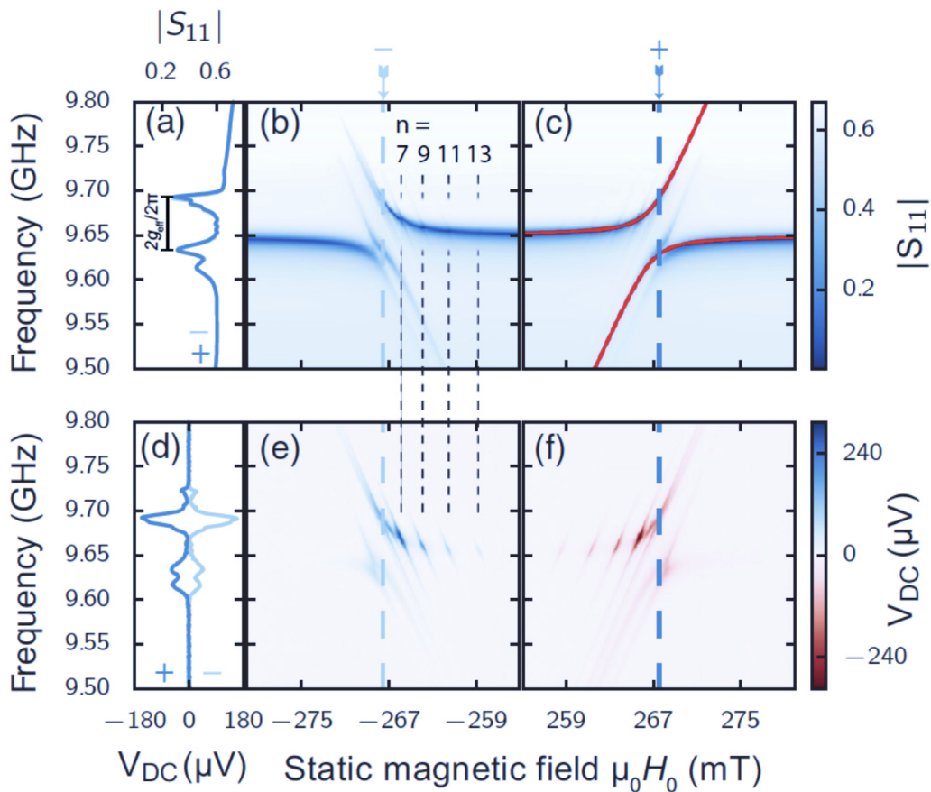
Fig. 12. (a), (d) Line cuts at H_0 = \pm 267.5 mT show the symmetry under field reversal for S_{11} (a) and V_{DC} (d). (b), (c) Reflection coefficient S_{11} recorded while sweeping the magnetic field and the MW frequency. Strong coupling of the collective spin excitations is indicated by a clear anticrossing, and spin wave modes to the low field side of the main resonance are visible. (e), (f) Simultaneously recorded dc voltage. The strongest signal is from the Kittel mode. Higher magnons modes are visible as well, however, they couple less strongly to the cavity. Source: Adapted from Maier-Flaig et al. [168]. Copyright by the American Physical Society.
