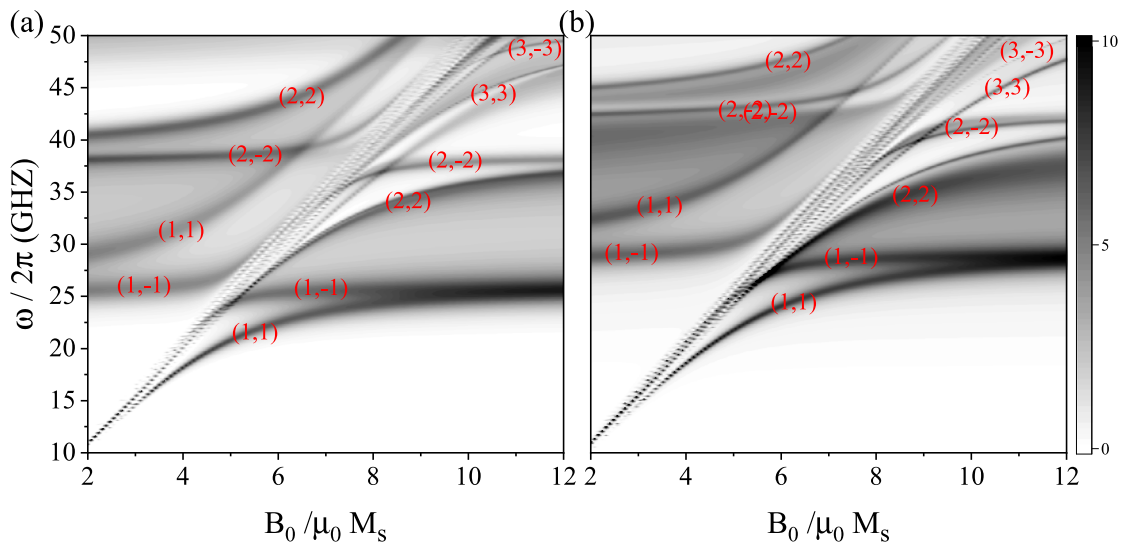
Fig. 9. Calculated scattering efficiency of a YIG sphere for the same parameters as Fig. 8, as a function of magnetic field B_0 and frequency, (a) with and (b) without the cavity. The MW modes are labeled by the spherical harmonic indices (n, m) . Source: Adapted from Zare Rameshti et al. [145]. Copyright by the American Physical Society.
