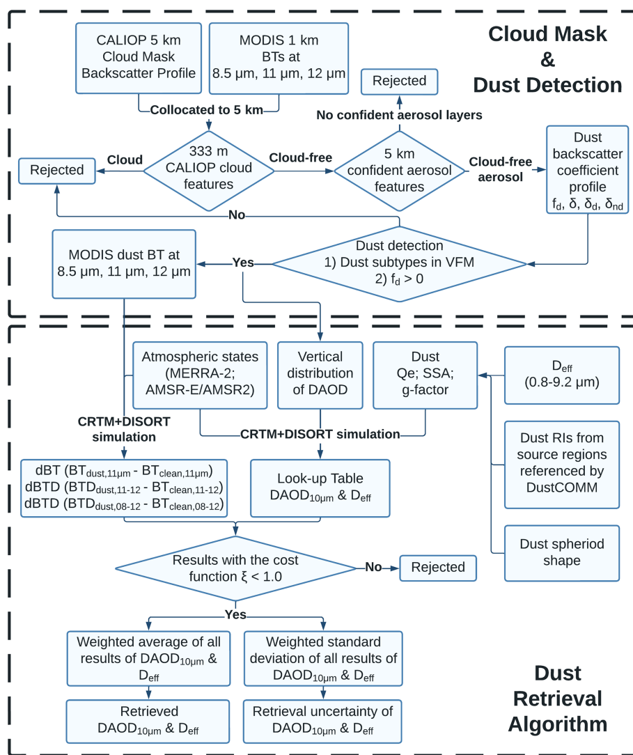
Figure 1. A flowchart of the retrieval process of \text{DAOD}_{10\mu\text{m}} and D_{\text{eff}} using collocated MODIS–CALIOP observations.
