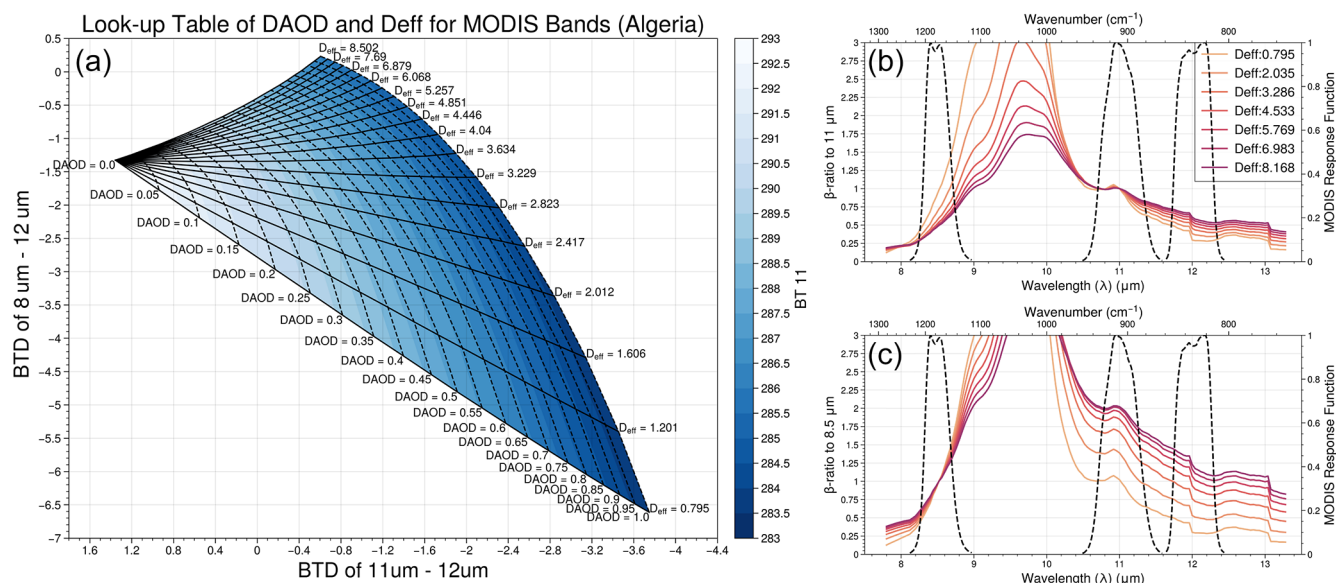
Figure 2. (a) An example of the LUTs of \text{BTD}_{8-12} (y axis), \text{BTD}_{11-12} (x axis) and \text{BT}_{11} (color-filled contours) corresponding to \text{DAOD}_{11\mu\text{m}} ranging from 0.0 to 1.0 (dashed lines) and D_{\text{eff}} ranging from 0.8 to 8.2 \mu\text{m} (solid lines) and the Algerian dust RI from the Di Biagio database. At the point of \text{DAOD} = 0.0 , the \text{BTD}_{8-12} and \text{BTD}_{11-12} correspond to the cloud-free clean scenario. (b) The \beta ratio to 11 \mu\text{m} calculated based on D_{\text{eff}} ranging from 0.8 to 8.2 \mu\text{m} and the Algerian dust RI within the TIR spectrum between 7.5 and 13.5 \mu\text{m} . (c) The same as (a) but the \beta ratio to 8.5 \mu\text{m} .
