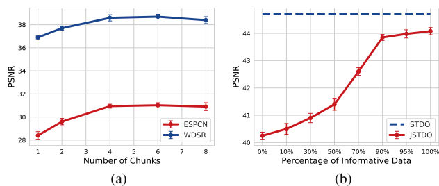
Figure 7. (a) PSNR of video game-15s on different number of chunks, (b) Comparison of different data schedule in joint training.
