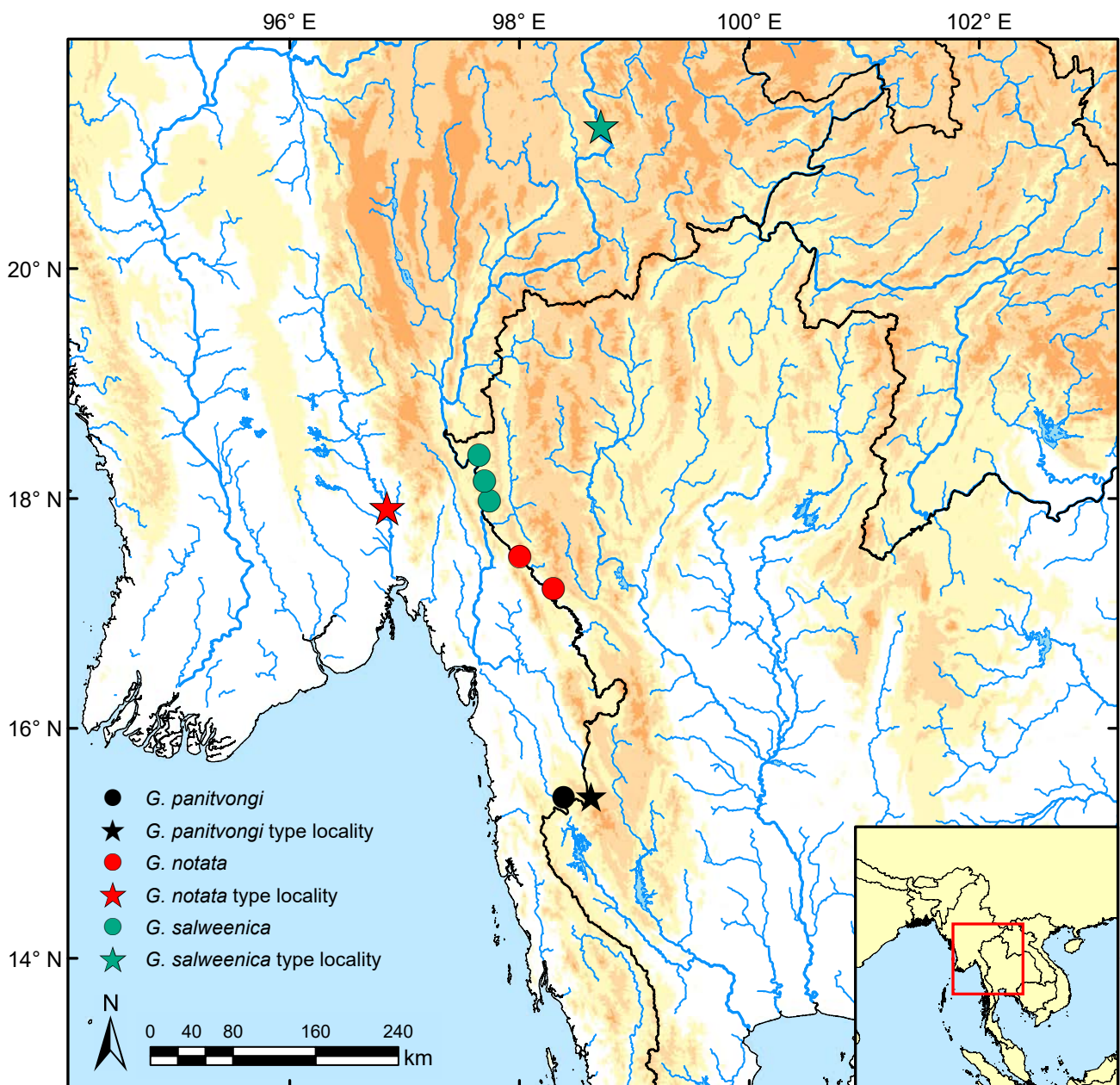
FIGURE 10. Distribution of specimens examined for this study and type localities of Garra notata and G. salweenica .
