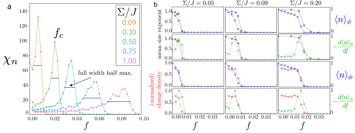
FIG. 14. Metrics for observing the condensation transition a \chi_n measured from simulations with \Phi = 0.1 , \Sigma/J \in 0.09, 0.3, 0.5, 0.75, 1.0 and fixed \beta\Sigma = 3.6 . The location of the peak of each distribution is used to identify the critical condensation frustration for the corresponding value of \Sigma/J and the full width half maximum is used as a measure of the uncertainty. b Comparison of the different metrics used to observe the condensation transition for the three values of surface energy to elastic (spin) stiffness ( \Sigma/J = 0.05, 0.09, 0.20 and \Phi = 0.15 ) used as examples Fig. 9bc. The peak of the mean size susceptibility (green) lines up with the point where both the mean size exponent (black) and the normalized charge density (red) drop to zero; hence we use the location of this peak to define the critical value of frustration.
