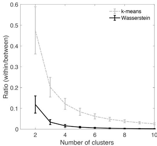
Fig. 13. The ratio \psi_i of the within-cluster distance over the between-cluster distance. The topological approach using the Wasserstein distance usually gives far smaller ratio compared to the traditional k -means clustering. In the elbow method, the largest slope change occurs at k = 3 and we determine k = 3 is the optimal number of clusters.
