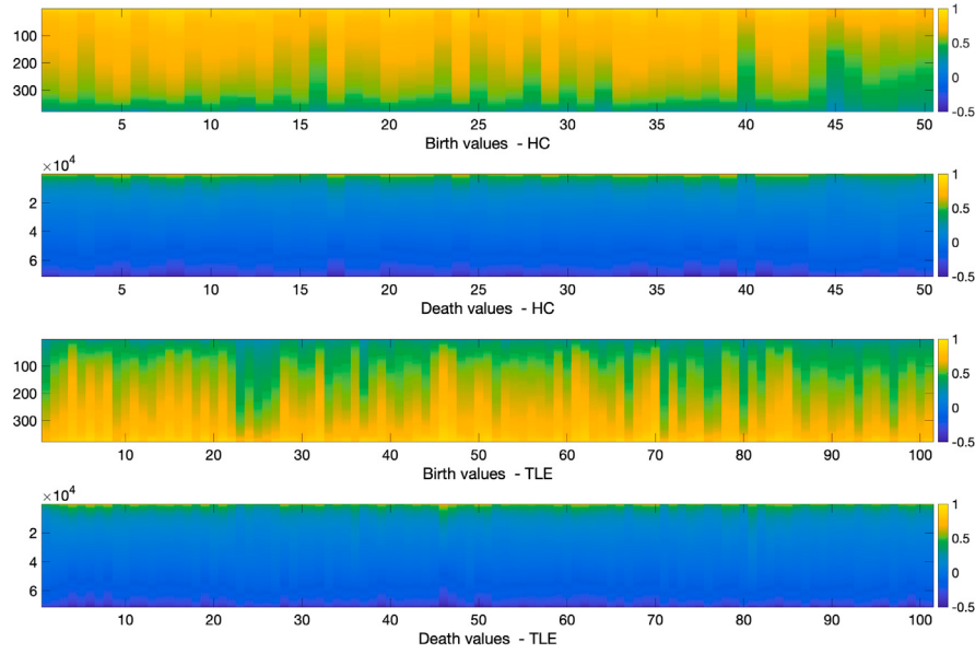
Fig. 5. The birth and death sets of 50 healthy controls (HC) and 101 temporal lobe epilepsy (TLE) patients. The Wasserstein distance between the birth sets measures OD topology difference while the Wasserstein distance between the death sets measures 1D topology difference.
