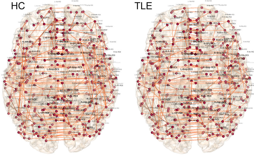
Fig. 6. Maximum spanning trees (MST) of the average correlation of HC and TLE. MST are the OD topology while none-MST edges not shown here are 1D topology. MST forms the birth set. MST of rs-fMRI is mainly characterized by the left-right connectivity.
