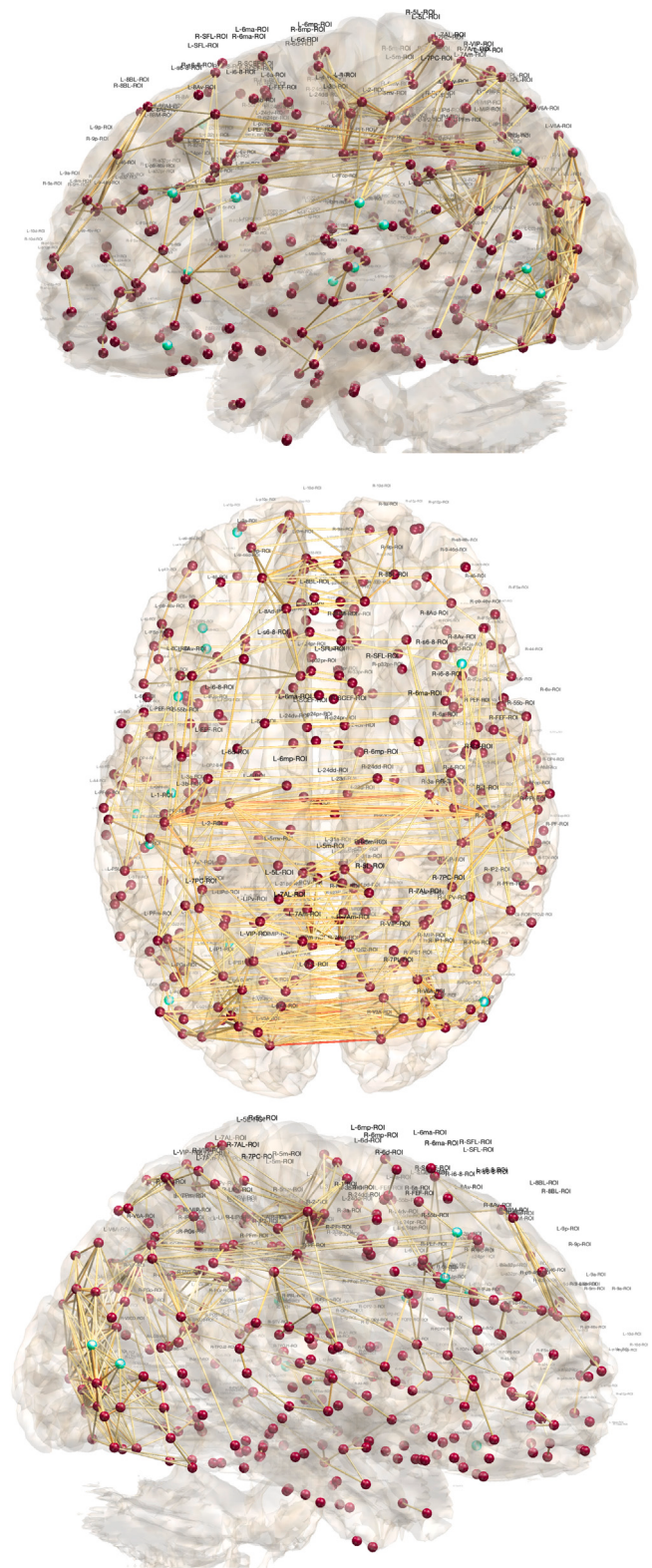
Fig. 12. 20 localized brain regions (teal color) identified under node attack on the ratio statistic \phi_L displayed over Glasser parcellated brain regions. The results are overlaid on top of average correlation map of TLE patients.
