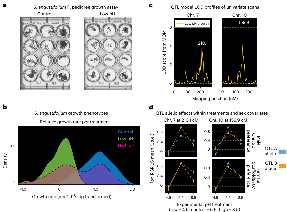
Fig. 5 | S. angustifolium pedigree QTL mapping in response to pH stress.
