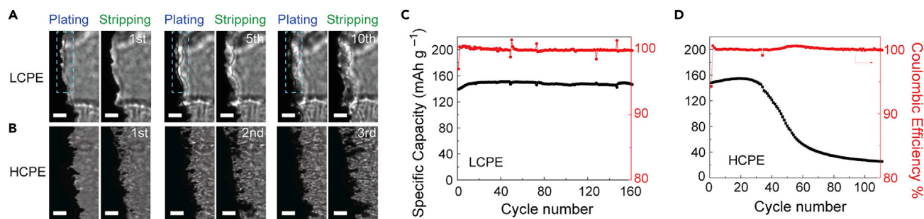
Figure 6. Cycling stability of the lithium metal anode in Li/Li cells and LFP/Li cells with PC/LiDFOB-LiBF 4 dual salt-based LCPE and HCPE (A and B) The bright-field images of the lithium electrodes in Li/Li cells with (A) LCPE and (B) HCPE at room temperature and 0.75 mA cm -2 . The scale bars are 25 μm to better show the as-formed new PEO-rich phase (the dashed blue area). (C and D) The cycling performance of LiFePO 4 /Li metal batteries with (C) LCPE and (D) HCPE at 38°C. The current density is 0.3 mA cm -2 . In LCPE, PEO:LiDFOB:LiBF 4 = 12:1:1, and PC is 90 wt % of PEO. In HCPE, PEO:LiDFOB:LiBF 4 = 6:1:1, and PC is 90 wt % of PEO.
